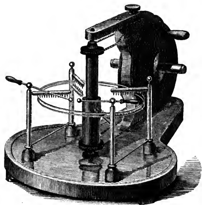
FIG. 8.—Holtz's Machine with Horizontal Plates.
