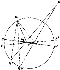
Fig. 14.—Duration of Spark.
