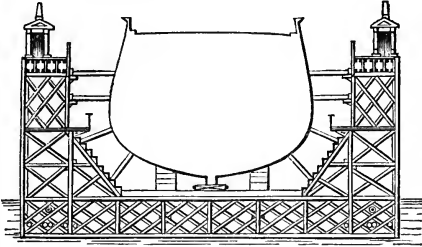
FIG. 6.—Transverse Section of Rennie's Floating Dock.
