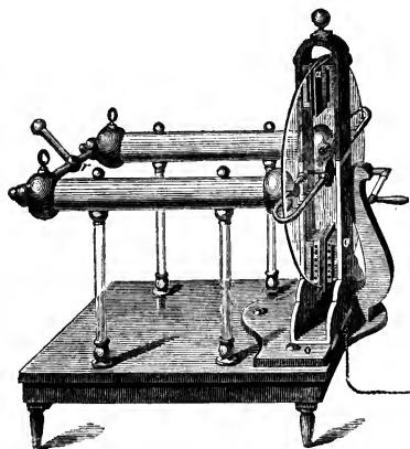
FIG. 6.—Ramsden's Plate Electrical Machine.
