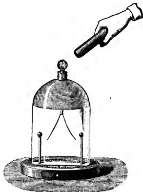
Fig. 3.—Bennet's Gold-leaf Electroscope.
