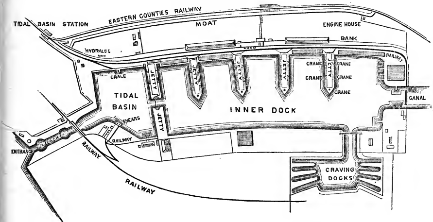
FIG. 1.—Plan of the Victoria Docks at London.
