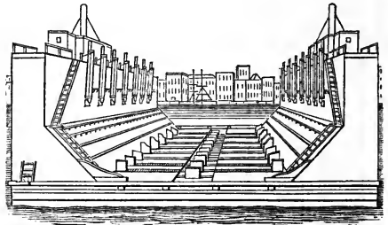
Fig. 5.—Balance Dock.
