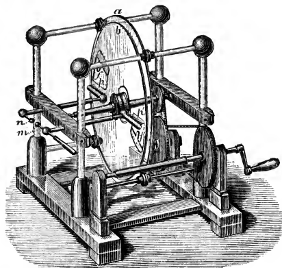
FIG. 7.—Holtz's Electrical Machine.
