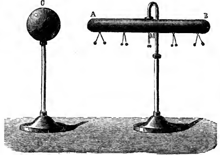
FIG. 2.—Electrification by Induction.
