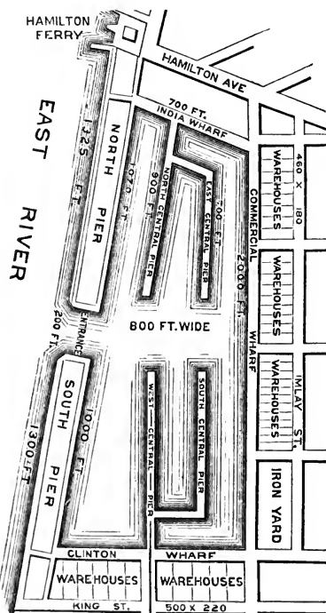
Fig. 2.—Plan of Atlantic Dock.
