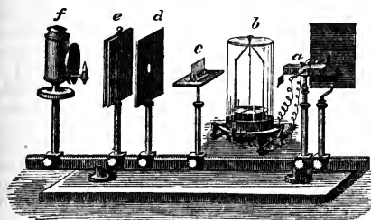
Melloni's Apparatus.
