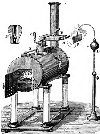
FIG. 10.—Sir William Armstrong's Hydro-electric Machine.
