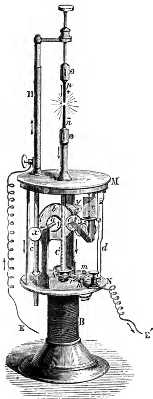
Duboscq's Regulator.
