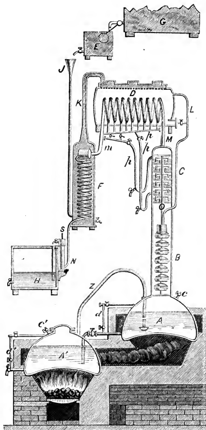
FIG. 4.—Derosne's Still.
