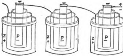
FIG. 16.—Coupling for Intensity.
