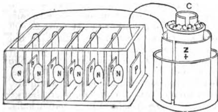
FIG. 81.—Compound Bath.
