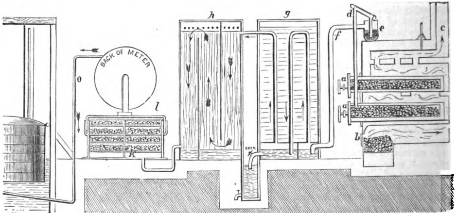
FIG. 7.—Synoptical Plan of Gas Works.
