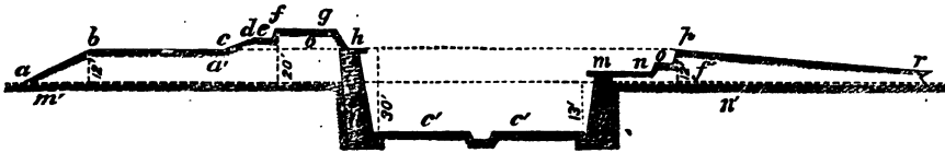
FIG. 1.— a , the rampart, of which ab is the slope, and bc the terreplein; b' , the parapet, of which cd ef gh is the outline; c'c' , the main ditch; d' , the scarp wall; e' , the counterscarp wall; f' , the embankment of the covered way, of which m'n is the terreplein, n'o p the outline of the banquette and interior slope, and p'r the glacis; m'n' , the natural surface of the ground; f' , the interior crest; g'h , the superior slope; g'h , the exterior slope; f'a , the interior slope; d'a , the banquette tread; c'a , the banquette slope.
