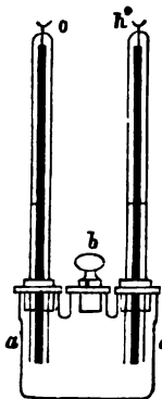
FIG. 29.—Gas Battery.
