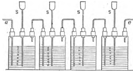
FIG. 4.—Woulfe's Bottles.
