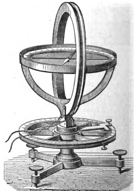
FIG. 19.—Sine Galvanometer.
