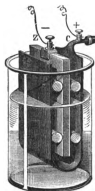
FIG. 5.—Cell of Wollaston's Battery.
