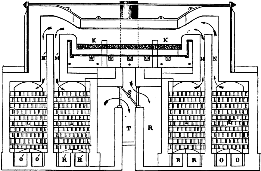
FIG. 5.—Siemens's Furnace.
