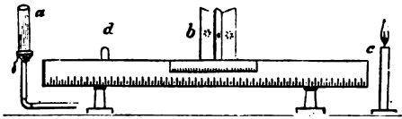
Fig. 8.—Bunsen's Photometer.
