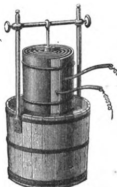
FIG. 6.—Hare's Calorimotor.
