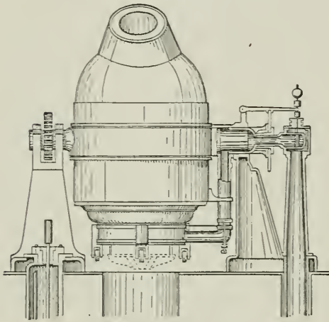
BESSEMER CONVERTER
