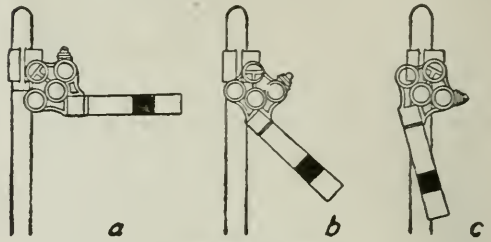
SEMAPHORE
