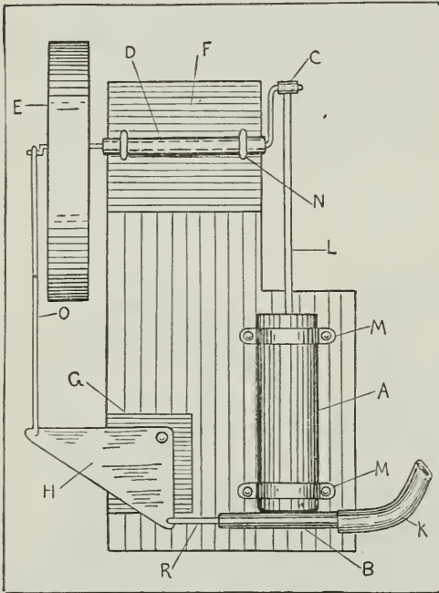
TOY STEAM ENGINE (Fig. 1)
