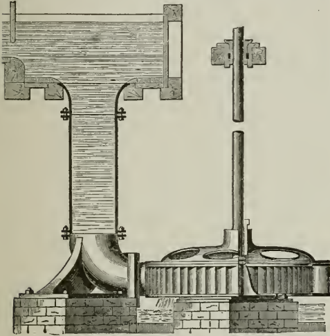
TURBINE WHEEL
