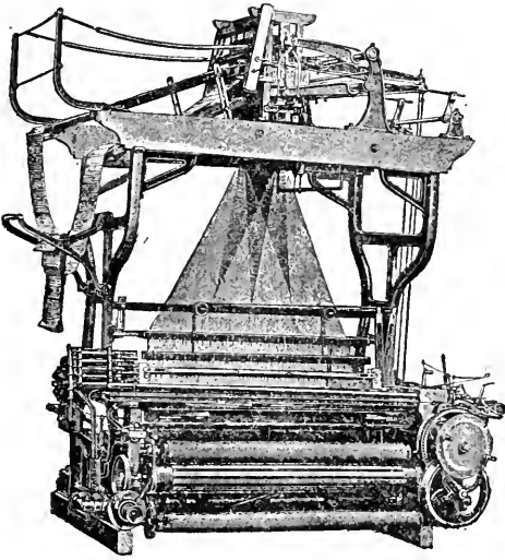
JACQUARD LOOM
