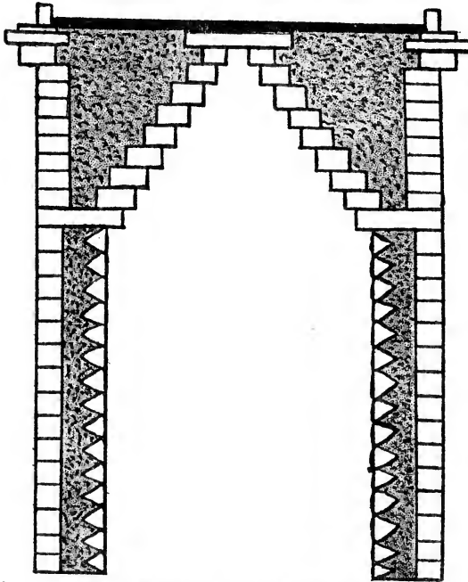
DIAGRAM OF MAYAN ARCH.
