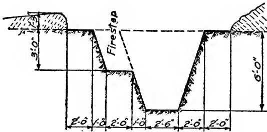
CROSS SECTION OF TRENCH (With Firestep)
