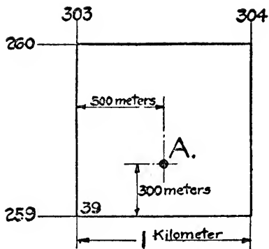
FIG. 3.—INTER-ALLIED SYSTEM. Kilometer square enlarged. Point "A" is the same as shown on Figs. 1 and 2. Coördinates of Point "A" within Square V are Written V3593, a Point 20 Meters N. and E. of Point "A" would be V352932. A Point with Similar Figures May Occur Every 50 Kilometers.
