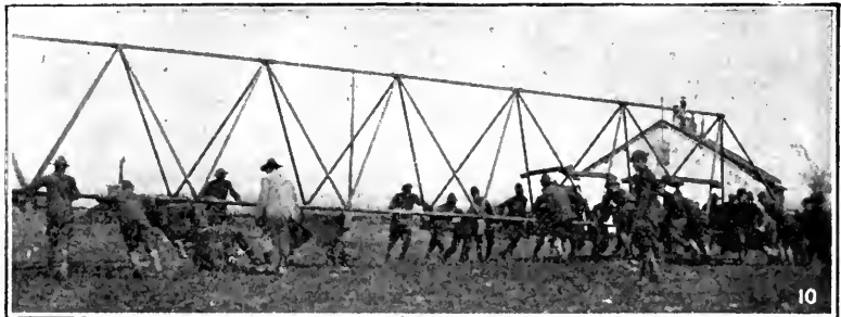
FIG. 7. THE FIRST BENT ERECTED AT ABOUT MIDDLE OF STRUCTURE, DIRECTLY OVER TWO-WHEEL TRUCK USED LATER FOR LAUNCHING
