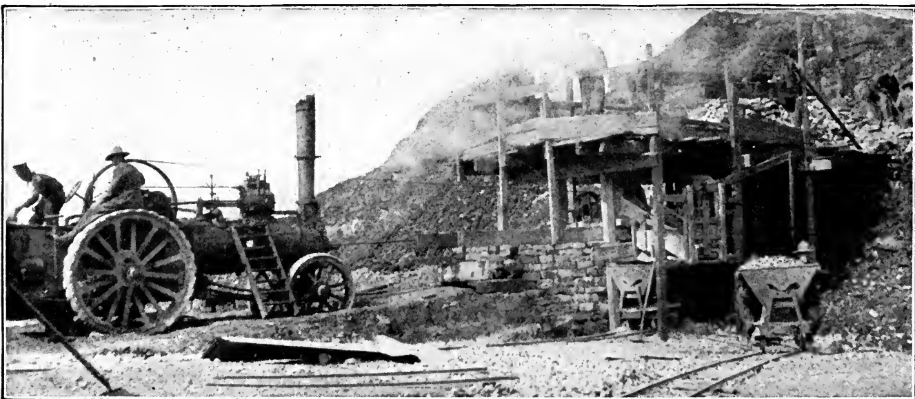
THIS QUARRY, TAKEN OVER FROM FRENCH, IS SHOWN PARTLY EQUIPPED WITH GYRATORY CRUSHER, THE OVERHEAD STORAGE BINS NOT HAVING BEEN BEGUN
