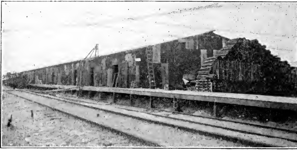
B. AFTER THE WOODEN FRAMEWORK WAS SET UP THE BUILDINGS WERE SHEATHED AND ROOFED WITH CORRUGATED IRON
