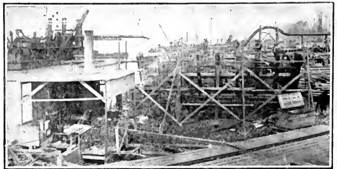
D. DREDGE PUMPING SAND FROM SCOW TO MAKE RAILROAD FILL—NOTE END OF ELEVATED PIPE LINE AT RIGHT, THROUGH WHICH SAND IS PUMPED
