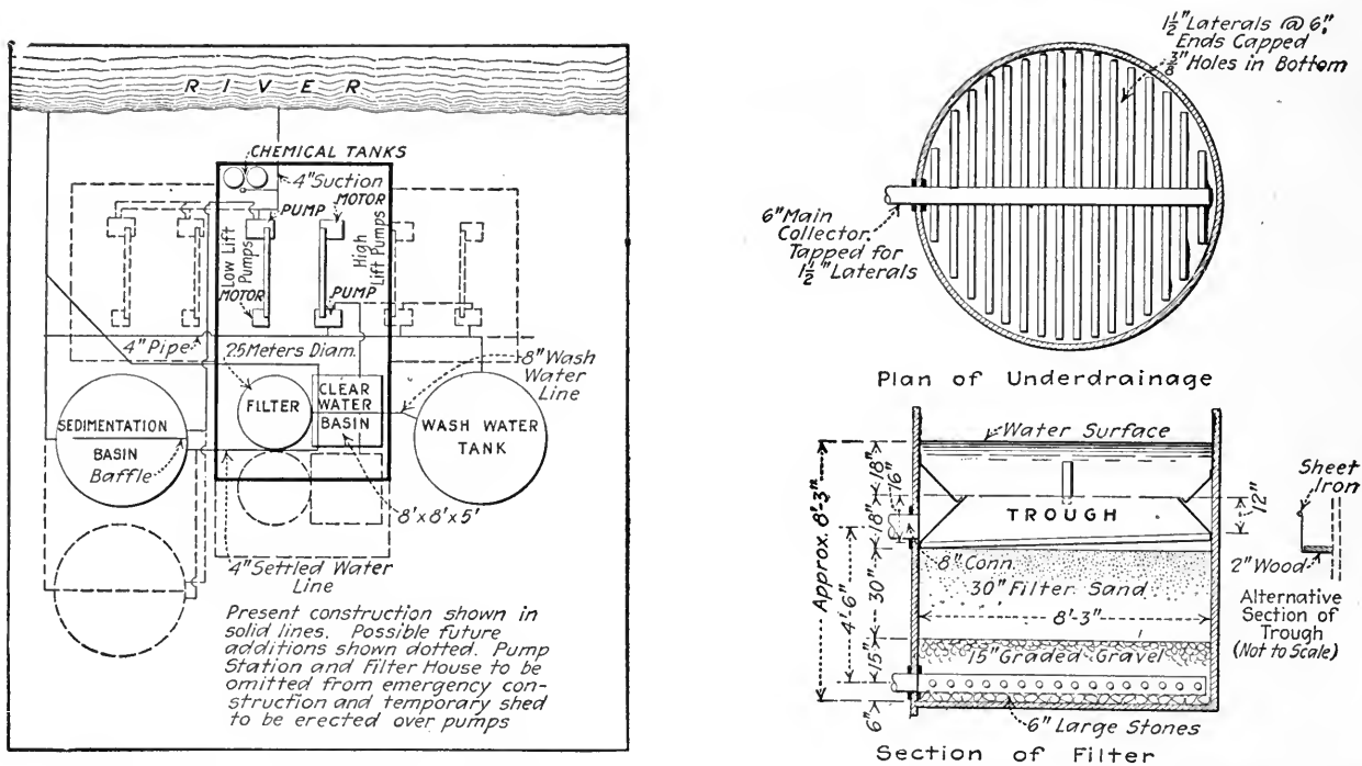
FIGS. 1 AND 2. DETAILS OF FIRST MECHANICAL FILTRATION PLANT BUILT BY AMERICAN ENGINEERS IN FRANCE
