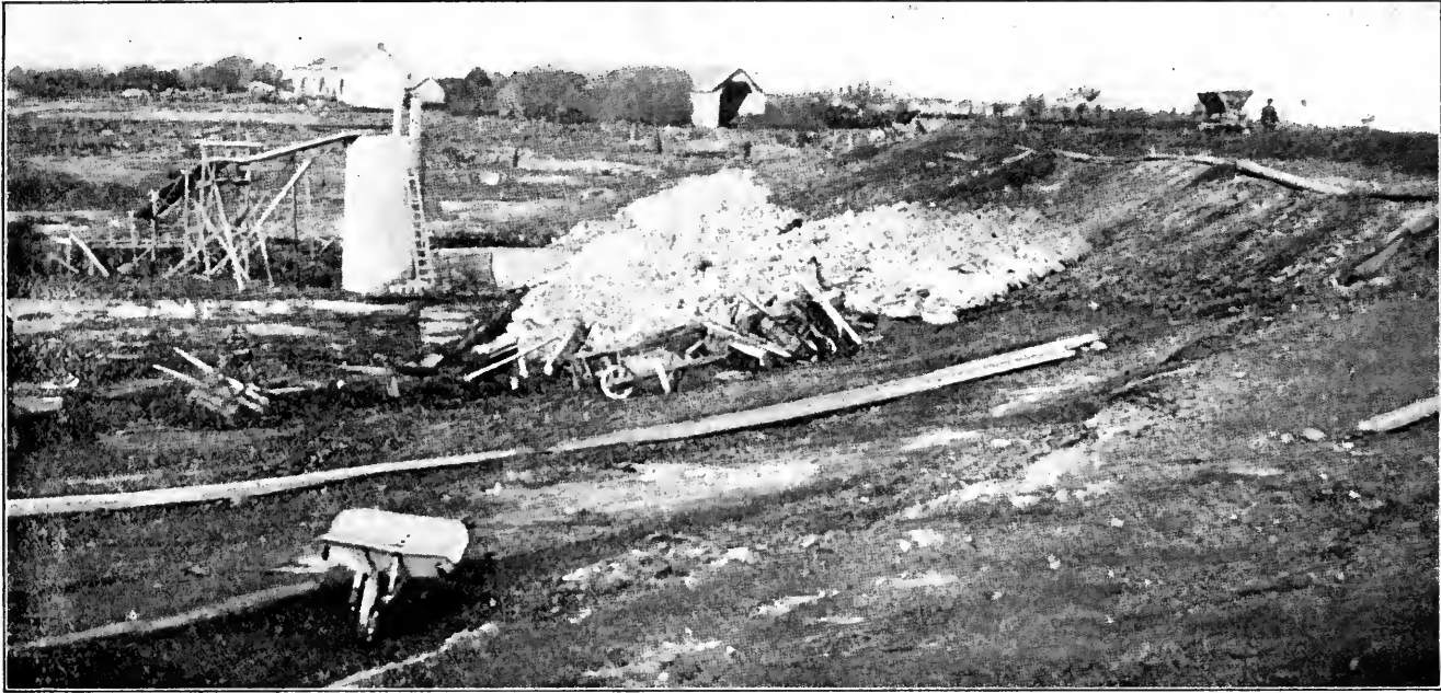
THIRTY-THOUSAND YARD EARTH DAM AT FRENCH SEAPORT BUILT WITH PICK AND SHOVEL
