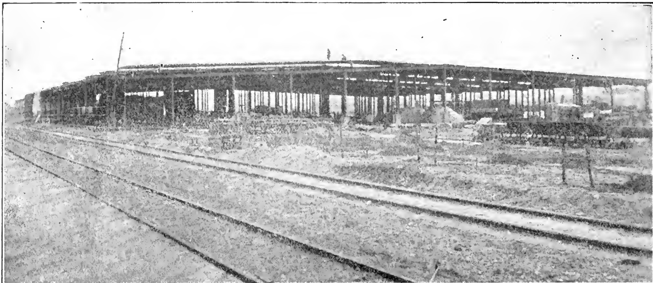
E. HOW ONE OF THE STEEL-FRAME ORDNANCE BUILDINGS, THE MACHINE SHOP, LOOKED ON APRIL 5
