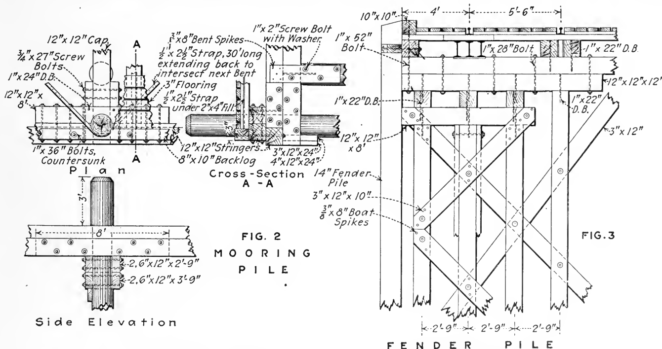
FIGS. 2 AND 3. DETAILS OF THE MOORING PILE AND THE FENDER PILE
