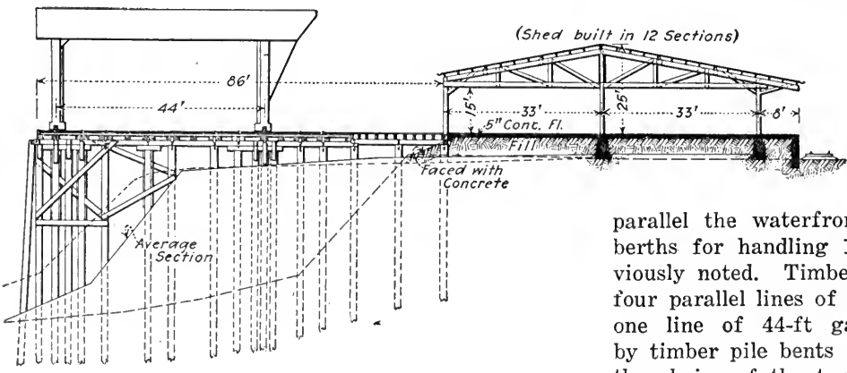
FIG. 1. CROSS-SECTION OF DOCK STRUCTURE AND CLASSIFICATION SHED
