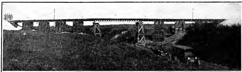
LIGHT RAILWAY CARS—OCCASIONALLY IT IS NECESSARY TO BUILD A TRESTLE
