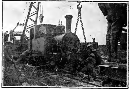
FIGS. 9 AND 10. WHEN THE HEAVIER STEAM LOCOMOTIVES ARE DERAILED, WRECKING CARS LIFT THEM BACK The lighter petrol tractors can often be handled by blocking, steel bars or rerailing irons
