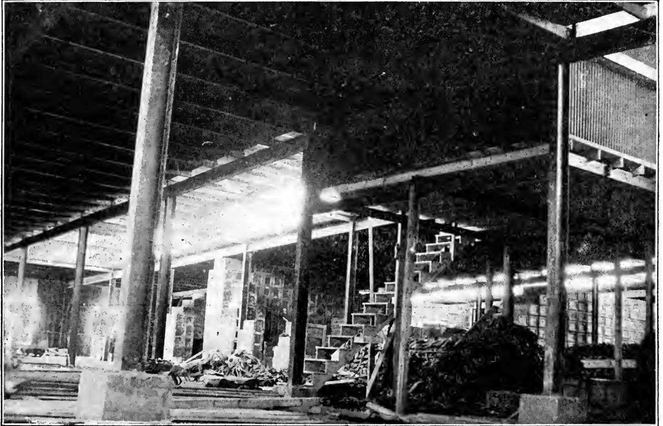
G. INTERIOR OF FINISHED ORDNANCE STORAGE BUILDING—COLUMNS SUPPORTED ON CONCRETE FOOTINGS OF DIFFERENT HEIGHTS TO GIVE SLOPE TO ROOF, SINCE ALL COLUMNS ARE OF SAME LENGTH
