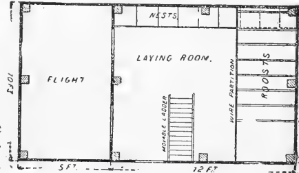
GROUND PLAN OF POULTRY HOUSE.
