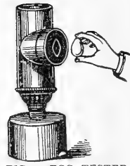
FIG. 3. EGG TESTER.
