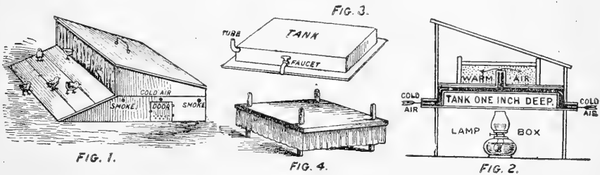
PLANS OF LAMP AND TANK BROODER.
