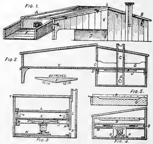
PLANS OF PRACTICAL BROODER
