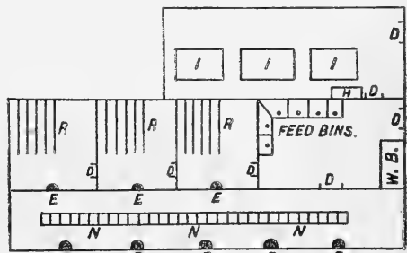
GROUND PLAN OF WELL ARRANGED HOUSE.
