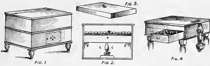
YOUTH'S COMPANION INCUBATOR.
