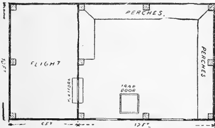
GROUND PLAN OF PIGEON LOFT.
