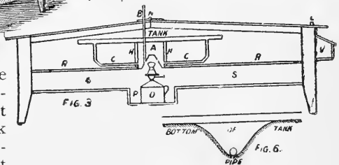
DETAILS OF TANK BROODER.
