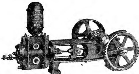
Fig. 708 horizontal double-acting power pump for operation by gasoline engine or electric motor. Good for 100 lbs. pressure.
