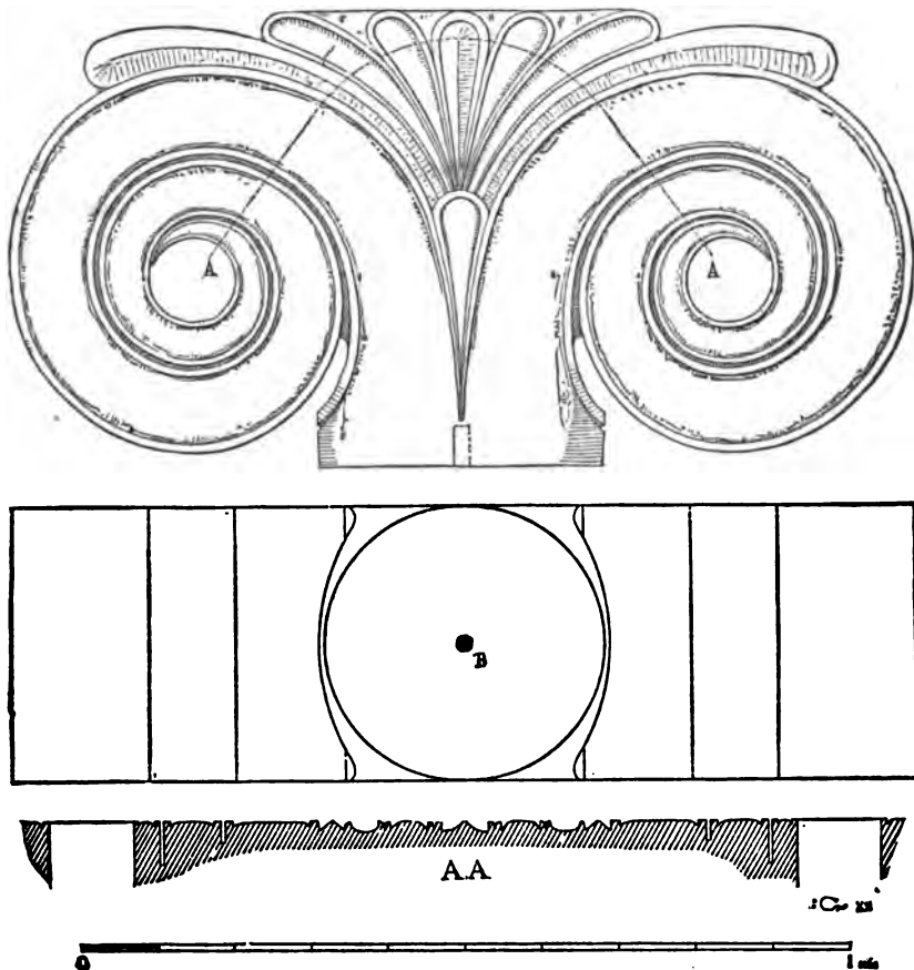
FIG. 2.—Restored view: plan and section of capital.
