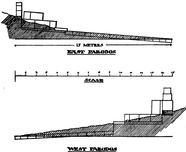
FIG. 38.—THE EAST AND WEST PARODOI.
