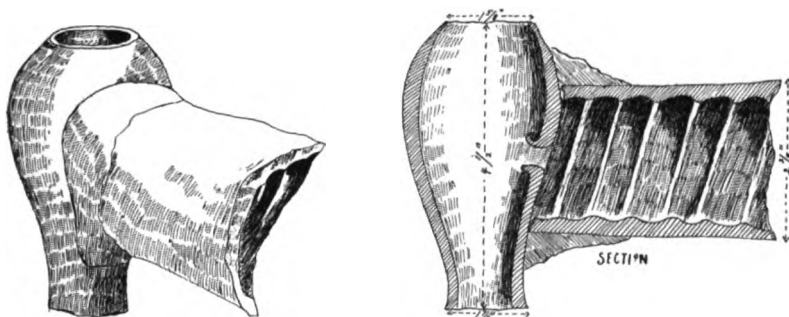
FIG. 21.—WATER VENT FORTY-FIVE FEET BELOW THE SURFACE S. E. OF THE ZIGGURAT.
