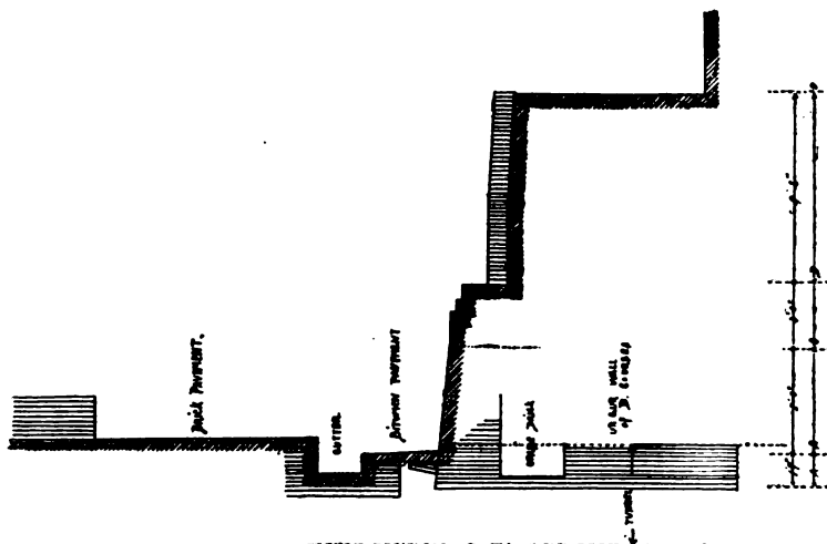
FIG. 18.—SECTION OF N. E. WALL OF ZIGGURAT, THIRTY FEET FROM E. CORNER. (Scale, .100 in. = 1 ft.)
