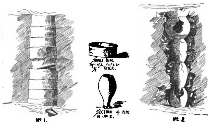
FIG. 13.—TERRACOTTA DRAINS FOUND IN MOUND No. 8.
