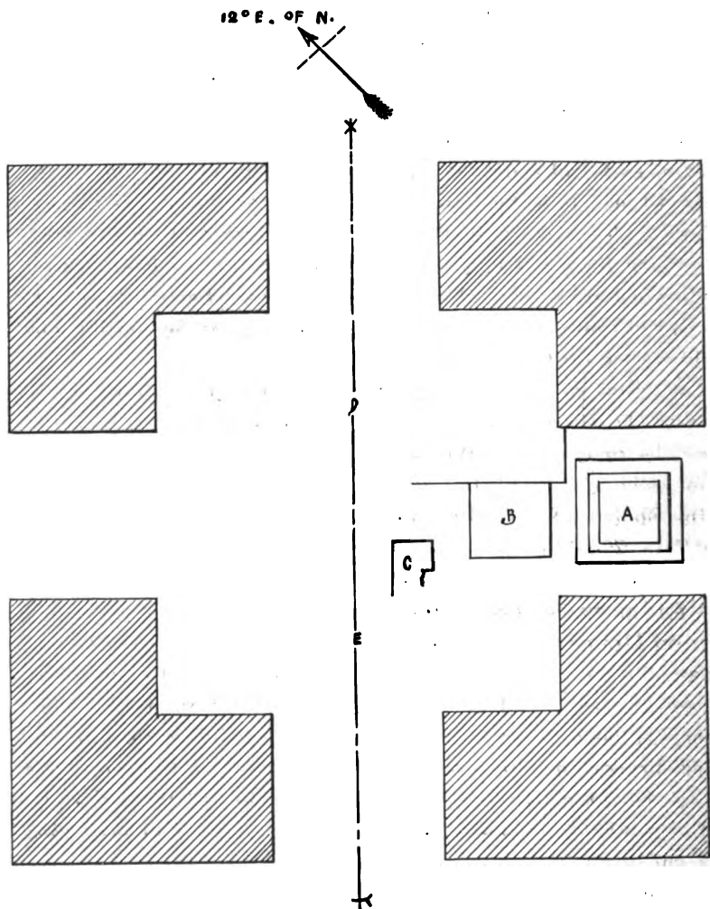
FIG. 63.—PLAN OF BUILDING OF BURNED BRICKS ON MOUND VI AT NIPPUR. SCALE .01088 M. = 1 M.
