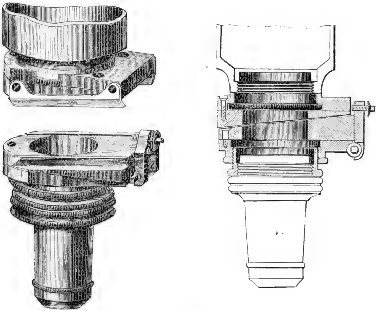
FIG. 3. — Zeiss Sliding Objective Changer.
