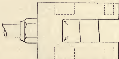
Fig. 45. Weak points in Crossheads.
