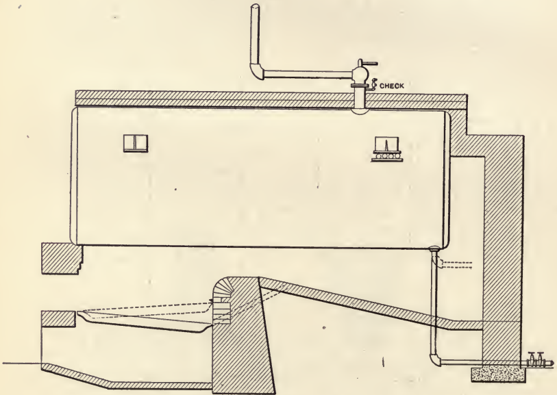
Fig. 14. Best Location of Blow-off pipe and valves.
