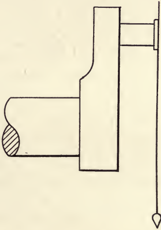
Fig. 60. Leveling shaft by plumb line.
