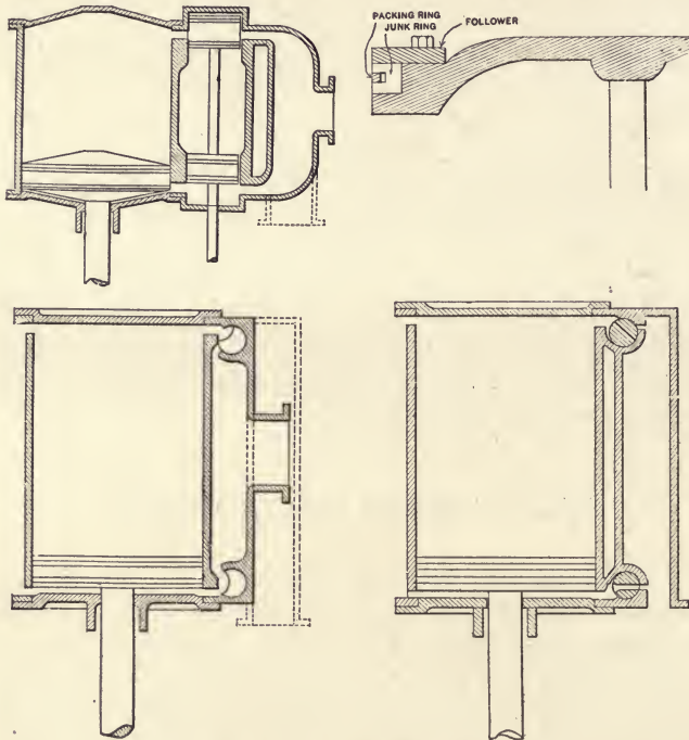
Figs. 63-65-66. Exhaust outlets.
