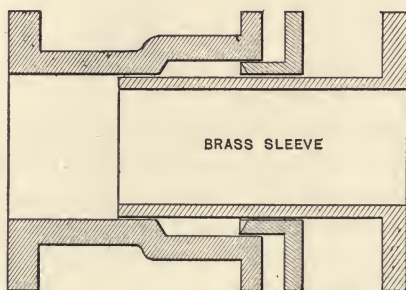
Fig. 35. A Slip Joint.
