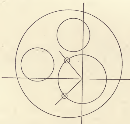
Fig. 81. Setting eccentric to reverse engine.
