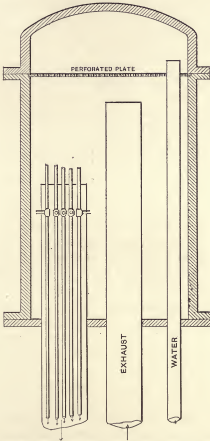
Fig. 85. The first syphon condenser—Ransom's.
