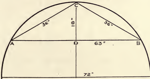
Fig. 99. Boiler calculations.
