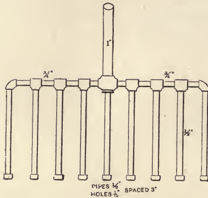
Fig. 3. A Home-made Blower.
