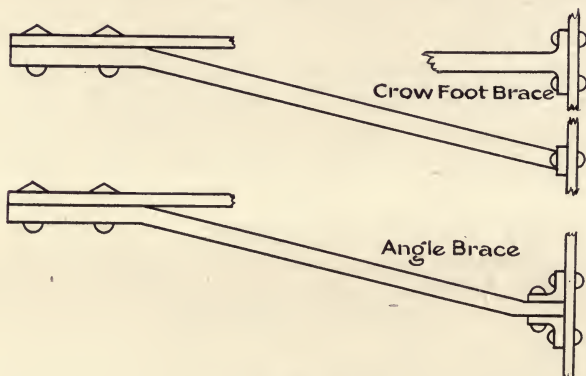
Fig. 104. Boiler braces.
