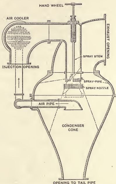
Fig. 87. Worthington's syphon condenser.
