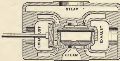
Fig. 82. Balanced slide valve.
