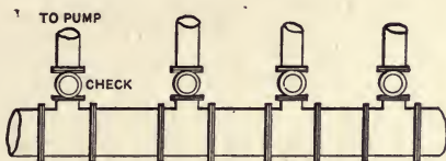
Fig. 36. Check Valves in Branch Pipes.
