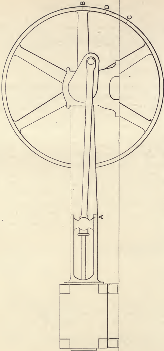
Fig. 77. Putting an engine on the center.
