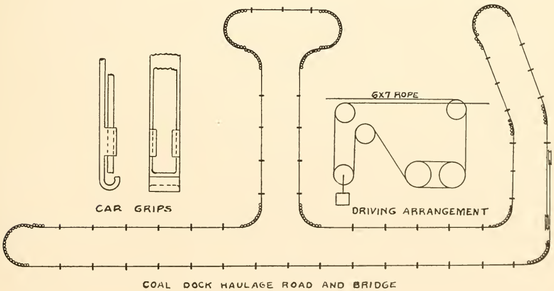
COAL DOCK HAULAGE ROAD AND BRIDGE
