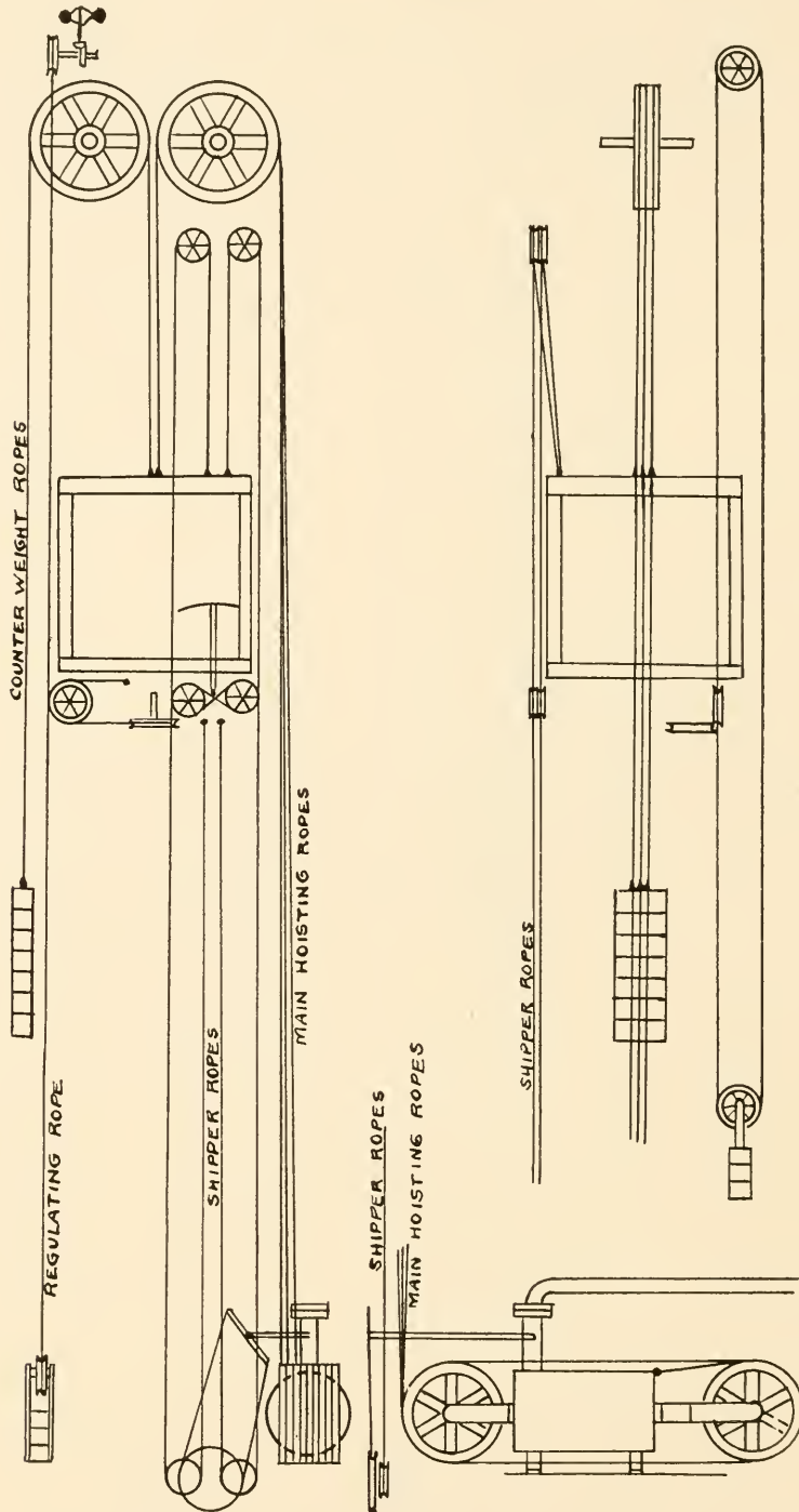
HORIZONTAL PLUNGER ELEVATOR
