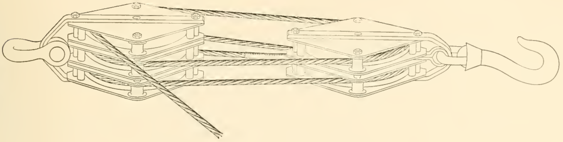
Five-part Line
