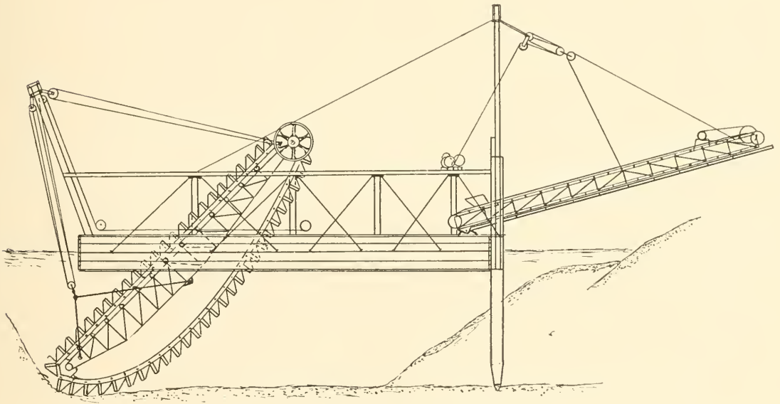
Bucket Ladder Dredge with Conveyor
