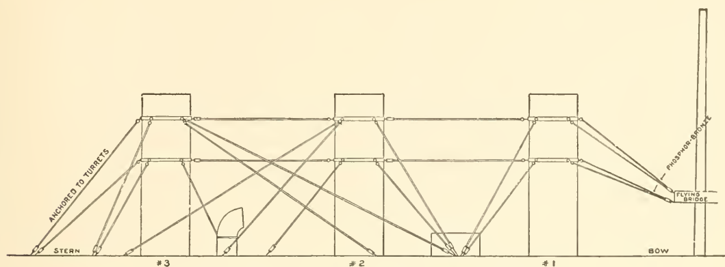
Plan of Smokestack Guys of U. S. Battleship Connecticut All guys of galvanized iron, 6 strands, 7 wires each, 2 1/2 inches circumference, 15,000 pounds strength
