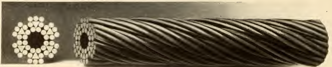
Type D—6 Strands 8 Wires—1 Hemp Core
