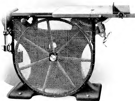
Wire Guard for Lower Wheel
