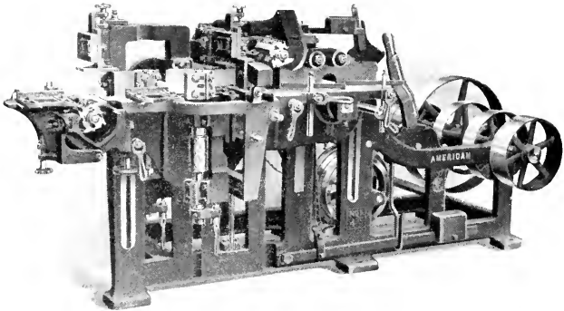
Figure 8641 American No. 1, 4" Four-sided Moulder
