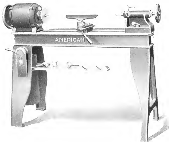
Figure 1064-C American 12-inch Speed Lathe With Motor Headblock and A. W. M. Special Control
