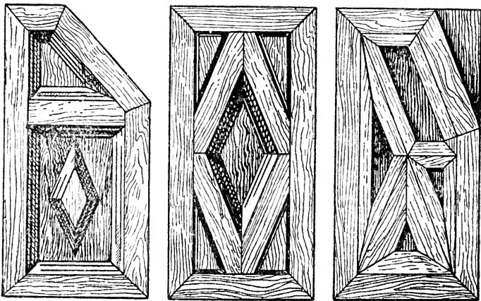
Panels made on the Universal Saw Bench with aid of the Protractor
