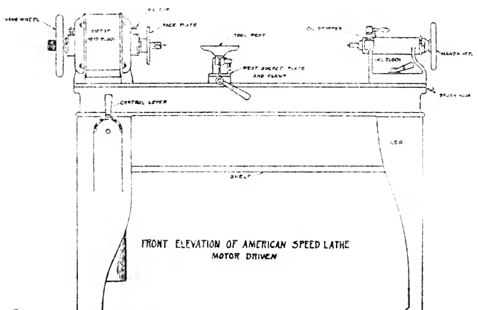
Front Elevation of Motor Headblock Lathe (American 12-Inch Speed Lathe)
