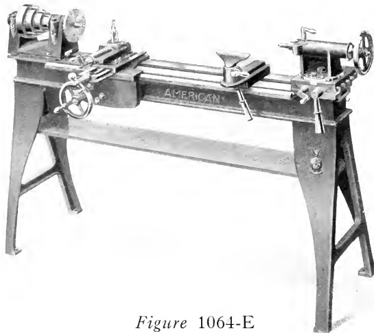
Figure 1064 American 12-inch Speed Lathe Plain with Countershaft
