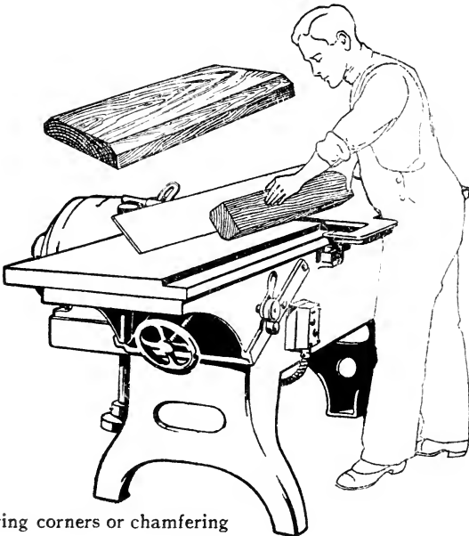
Planing out of Wind
