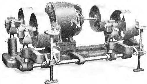
Special Motor Countershaft. As applied to Nos. 20 and 30.
