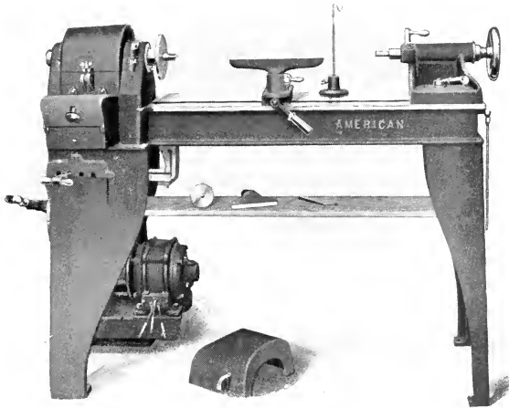
Figure 1064-D American 12" Speed Lathe A. C. Motor Mounted on Saddle and A. W. M. C. Enclosed Switch
