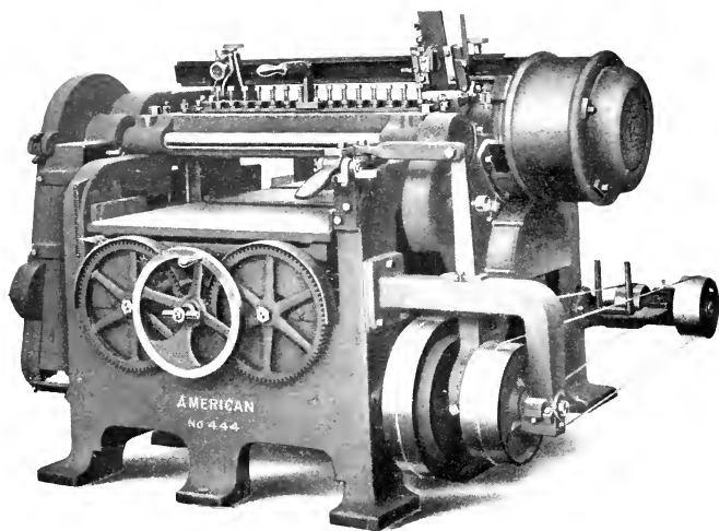
With Variable Feed and Direct-Attached Motor
