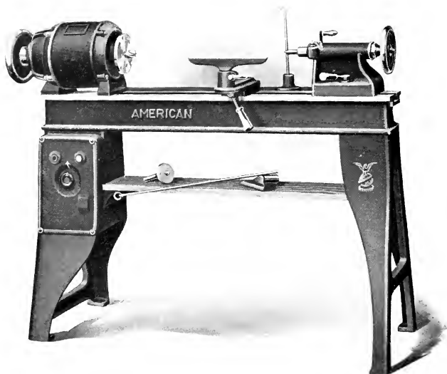
Figure 1064-B American 12-inch Speed Lathe With Motor Headblock and A. W. C. Special Control
