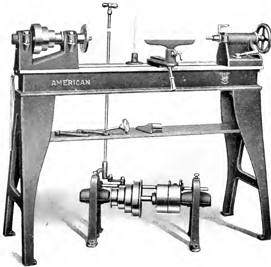
Figure 1064 American 12-inch Speed Lathe Plain with Countershaft
