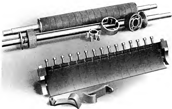
Sectional Feed Roll and Chipbreaker Applicable to No. 444 Surfacer
