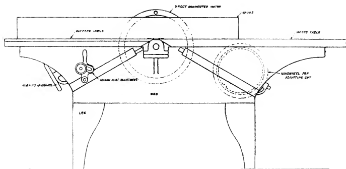
Front Elevation of Hand Jointer (American No. 1)
