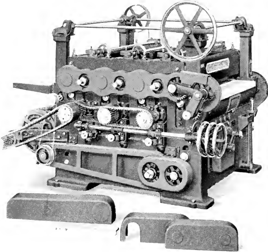
American No. 2 Columbia Three Drum Sander (Silent Chain Drive—Motor)
