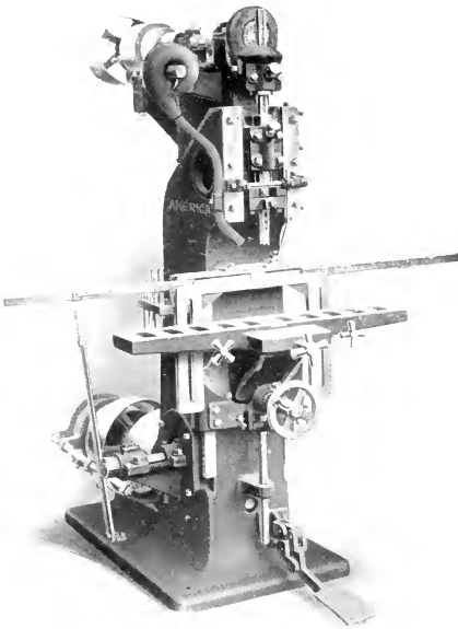
Figure 901—Plain Table
