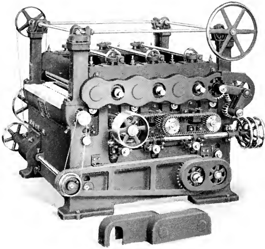
American No. 2 Columbia Three Drum Sander (Silent Chain Drive—Belt)
