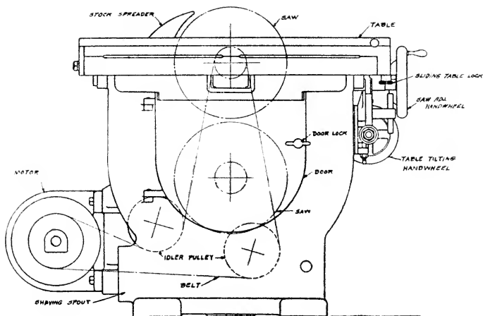
Front Elevation of Universal Saw (American No. 20 Universal Saw)
