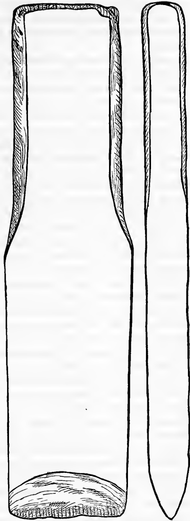
COPPER CHISEL. Full size.—Length 7\frac{1}{2} in.; breadth 1\frac{3}{4} in.; thickness \frac{3}{8} in. Minnesota Mine.
