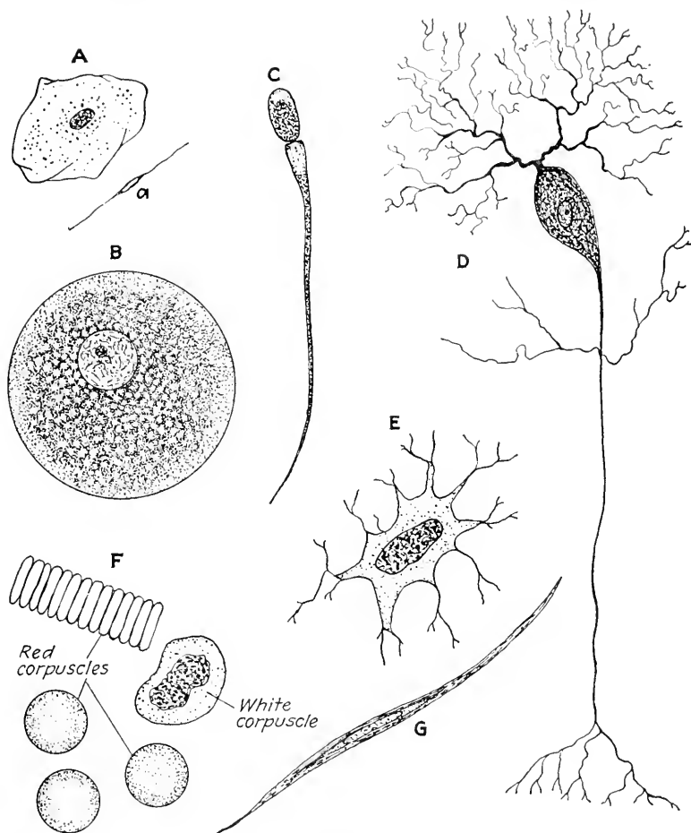
FIG. 4.— Various types of cells. A , epithelial cell shed from the lining of the human mouth; a is a side view of the cell. \times 300 . B , human ovum, nearly mature. \times 200 . C , human sperm cell. \times 1300 . D , diagram of a nerve cell. E , a bone cell; somewhat diagrammatic. \times 700 . F , human blood corpuscles. \times 1,000 . G , nonstriated muscle cell from mammalian intestine. \times 640 .
