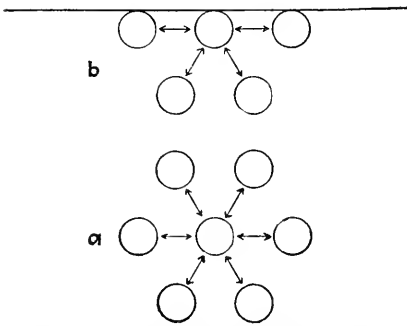
FIG. 1.—Diagram illustrating the balanced attraction exerted upon a molecule in a mass of liquid ( a ), and the unbalanced attraction upon a molecule at the surface ( b ). The two-pointed arrows ( \leftrightarrow ) indicate mutual attraction between two molecules.
