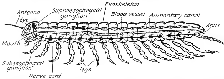
FIG. 200.—Diagrammatic representation of the structure of an arthropod. (From Schmil, "Text-book of Zoology," by the courtesy of A. and C. Black, and Quelle and Meyer.)
