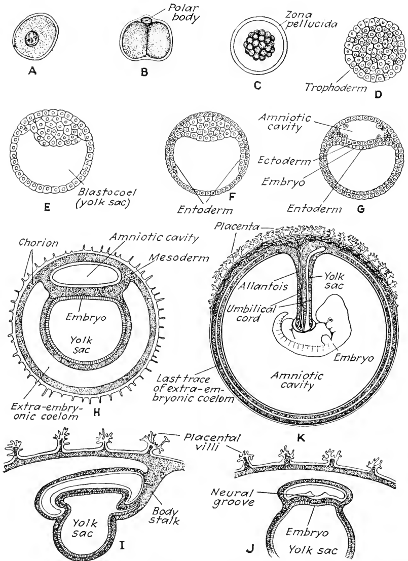
FIG. 287.—Diagrammatic representation of the stages in mammalian development. A, egg cell, in section. B, two-celled stage. C, morula. D, section of morula. E, blastula, in section. F, development of entoderm. G, formation of amniotic cavity, and separation of embryonic disc into entoderm and ectoderm. H, development of mesoderm and extra-embryonic coelom. I, formation of body stalk and beginning of placenta. J, cross section of same stage as I. K, embryo in amniotic cavity, the increase of size of which is about to obliterate the extra-embryonic coelom. In H to K, ectoderm is white, entoderm crosslined, and mesoderm stippled.
