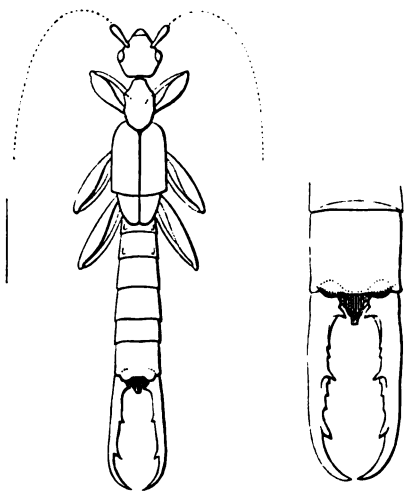
Psalidophora angusticollis ♂.
