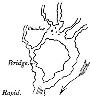
Whirlpools of the Chambal.
