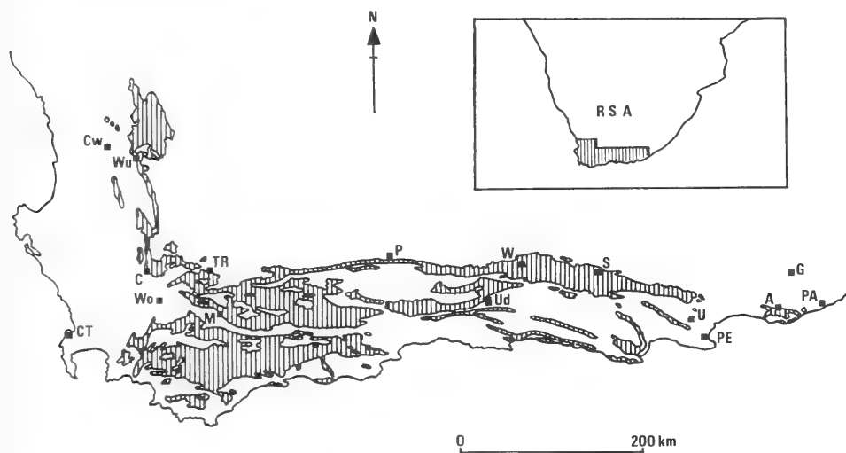
Fig. 2. Map showing the outcrop of the Bokkeveld Group rocks in the Cape Province and indicating the positions of towns mentioned in the text. A—Alexandria, C—Ceres, CT—Cape Town, Cw—Clanwilliam, G—Grahamstown, M—Montagu, P—Prince Albert, PA—Port Alfred, PE—Port Elizabeth, S—Steytlerville, TR—Touws River, U—Uitenhage, Ud—Uniondale, W—Willowmore, Wo—Worcester, Wu—Wuppertal.
