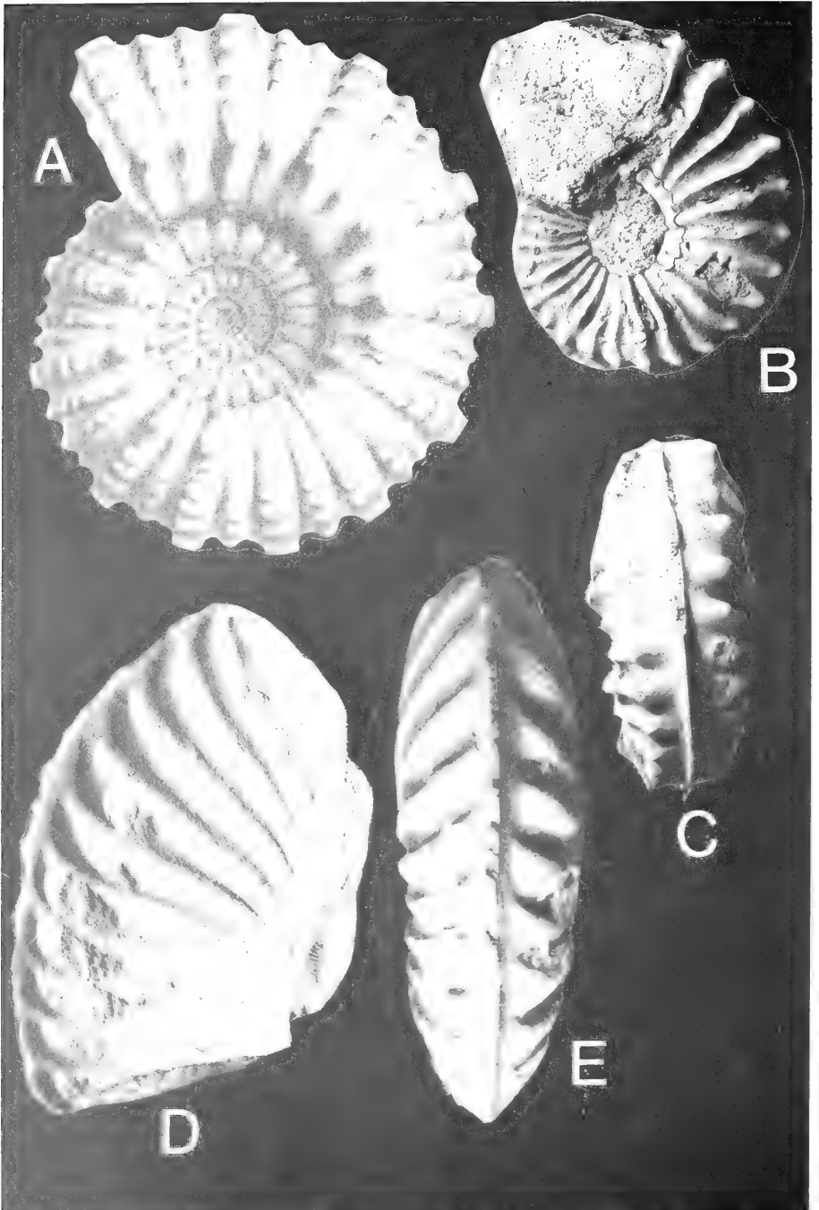
Fig. 22. A. Dowilleiceras variable Tavani, D'Orbigny's (1841, pl. 72 (fig. 5)) photograph, \times 0.5 . B-C. Mojsisoviczia delaruei (d'Orbigny), NHMP-5761, one of D'Orbigny's syntypes from Clar, France. D-E. Oxytropidoceras ( Mirapelia ) buarquianum (White), SAM-PCA2641, a rather densely ribbed douglasi morphotype, thus transitional to salasi variants. All \times 1 unless otherwise stated.
