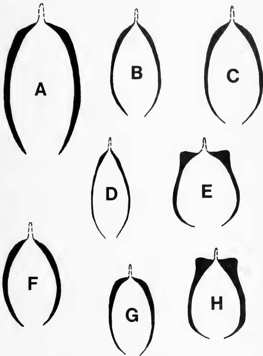
Fig. 23. A-D, F-G. Whorl sections of Oxytropidoceras (Mirapelia) buarquianum (White). A. SAM-PCA2656, a douglasi morphotype. B. SAM-PCA2644, a douglasi morphotype. C. SAM-PCA3603, a salasi morphotype. D. SAM-PCA2693, a typical buarquianum morphotype. F. SAM-PCA2622, a douglasi morphotype. G. SAM-PCA2641, a douglasi morphotype. E, H. Whorl sections of O. (M.) sergipense (White). E. SAM-PCA5444. H. An unnumbered specimen in the South African Museum. All \times 1 .
