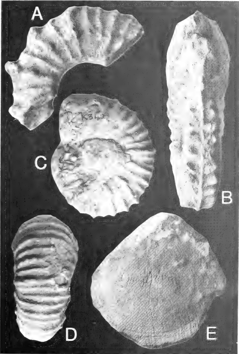
Fig. 11. A. Douvilleiceras inaequinodum (Quenstedt), SAM-PCA3458, a specimen showing the increased number of intercalatories in maturity. B. Oxytropidoceras (Mirapelia) sergipense (White). Front view of SAM-PCA5444. C-D. Douvilleiceras variabile Tavani, SAM-PCA3422. E. Plagiostoma sp., SAM-PCA5490, from the Oxytropidoceras assemblage. All \times 1 .
