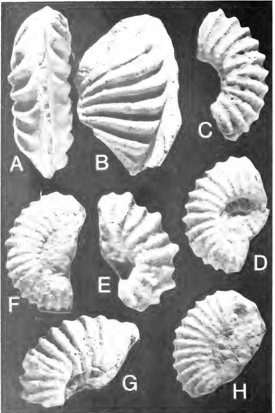
Fig. 10 A-B. Oxytropidoceras (Mirapelia) buarquianum (White). SAM-PCA2656, a douglasi morphotype which very closely approaches O. mirapelianum (d'Orbigny), \times 0.75 . C-D. F-H. Douvilleiceras mammillatum aequinodum (Quenstedt). C. SAM-PCA3494. D. SAM-PCA 3503. F. SAM-PCA3527. G. SAM-PCA3499. H. SAM-PCA3518. E. Douvilleiceras inaequinodum (Quenstedt). SAM-PCA3504. All \times 1 unless otherwise stated.
