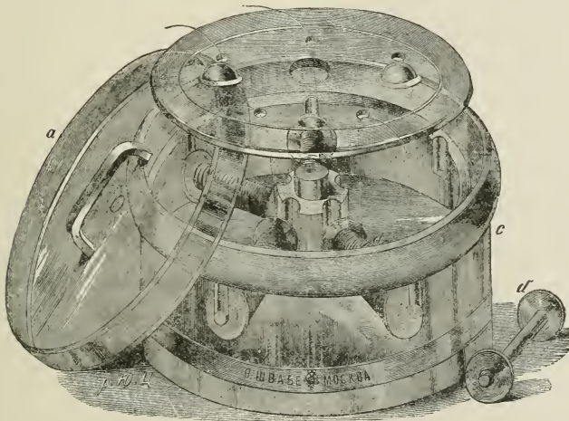
FIG. 2. LIGATURE JAR. Ready for use.
