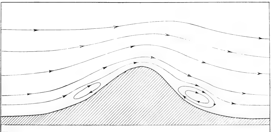
FIG. 2.—WIND EDDIES.
