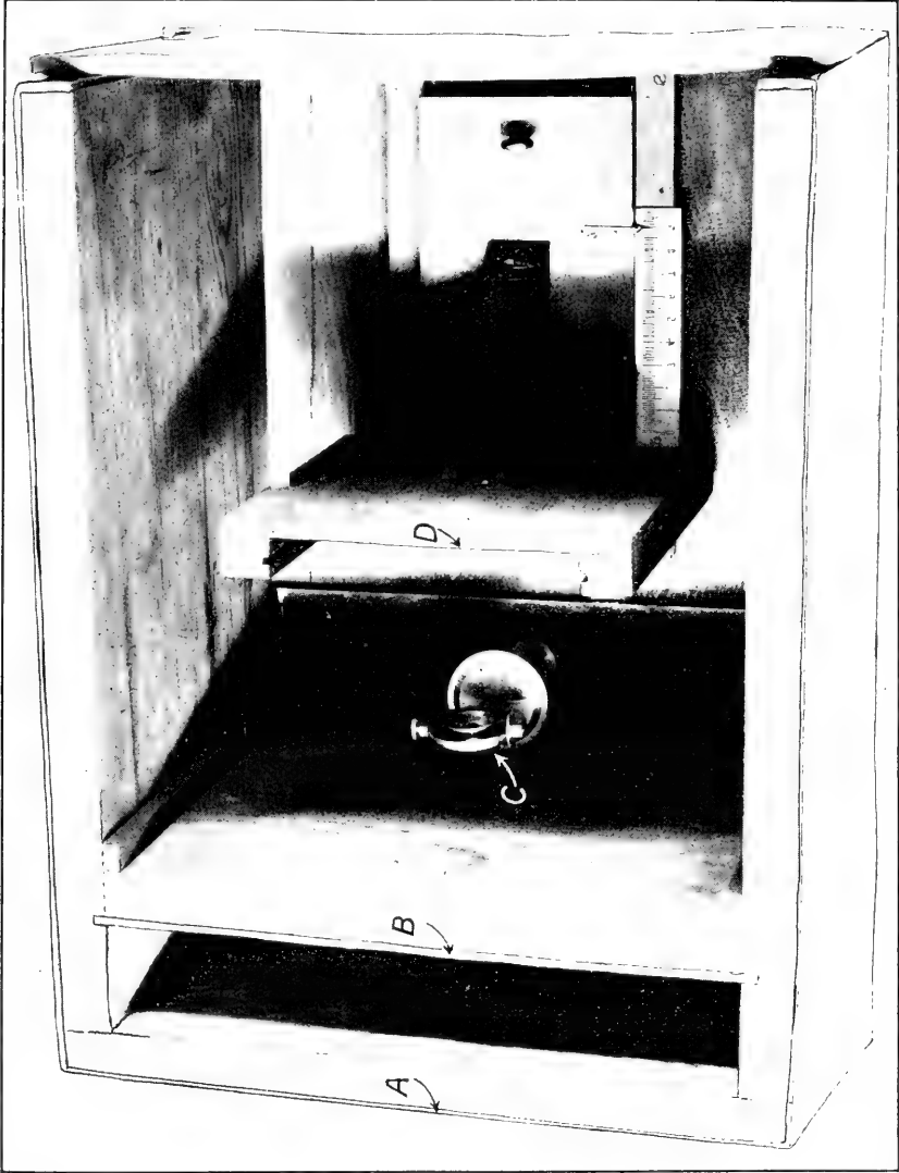
Fig. 20.—A form of the apparatus required for the preparation of Laue photographs. A and B are pinhole lead slits; the crystal holder C permits setting the section of the crystal at any desired orientation; D is a movable plate holder. Other and more complicated forms have been used; this one is desirable chiefly because of its simplicity.
