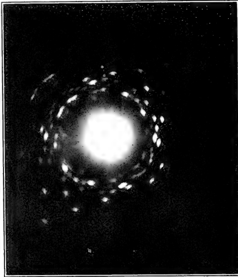
FIG. 4.—Potassium sulphate. Orthorhombic. X rays normal to the (001) face.
