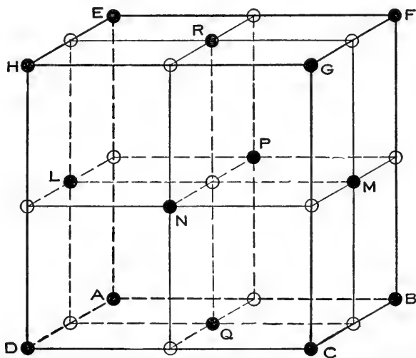
Fig. 22.—The sodium chloride arrangement. The black circles represent the positions of the atoms of one kind; the white circles those of the second kind of atoms. The alkali halides and the oxides of the divalent metals seem to have this atomic arrangement. Either the black atoms or the white ones have the grouping of the closest cubic packing of spheres.
