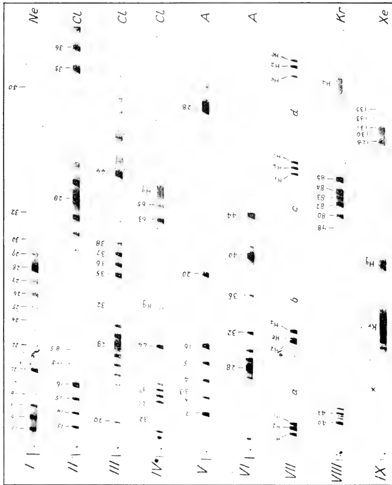
MASS SPECTRA OF VARIOUS CHEMICAL ELEMENTS.
