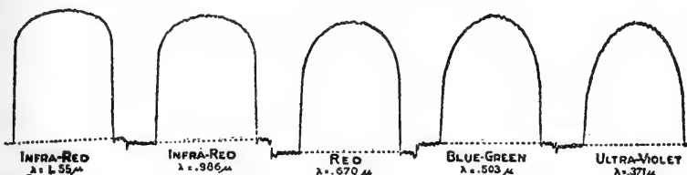
FIG. 2.—Brightness distribution along sun's diameter for different colors.
