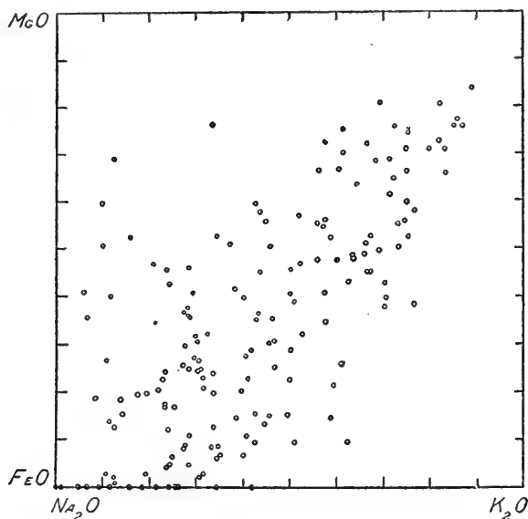
FIG. 1.—Relation of Na and Fe to K and Mg.
