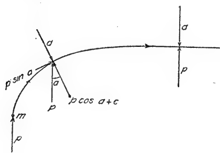
FIG. 1.—Diagram showing deflection of particle of air toward the east.
