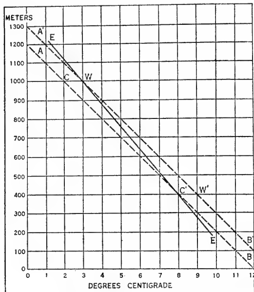
FIG. 2.—Vertical temperature gradients of free air.
