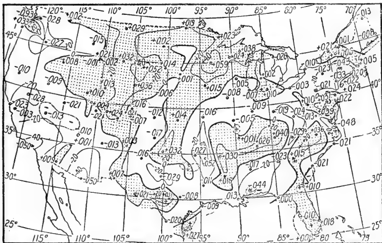
FIG. 6.—Dotted portions: Areas of positive anomaly, excess of mass. Due to surface too high or density of upper crust above mean. Blank portions: Areas of negative anomaly, deficiency of mass. Due to surface too low or density of upper crust below mean. Gravity anomalies in the United States.
