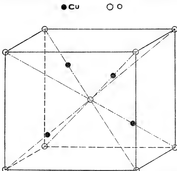
FIG. 23.—The cuprous oxide arrangement. Each monovalent copper atom is surrounded by two equally distant oxygen atoms and each divalent oxygen atom by four copper atoms. The white atoms alone have the body-centered grouping.
