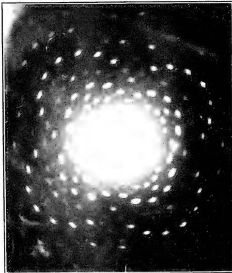
FIG. 5.—Rutile. Tetragonal. X rays normal to the (001) face.
