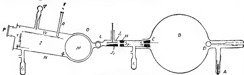
FIG. 2.—Diagram of the mass-spectroscope.
