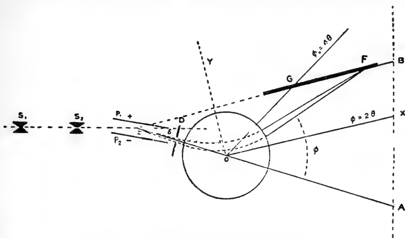
FIG. 1.—Theory of the mass-spectrocope.
