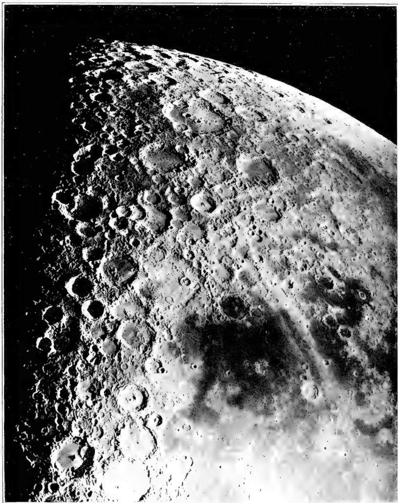
SOUTHERN PORTION OF THE MOON AT LAST QUARTER.
