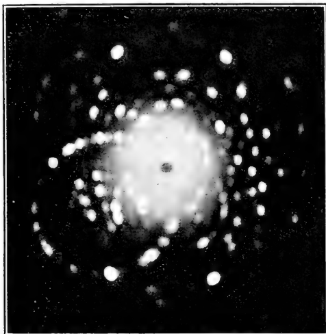
FIG. 2.—Cyanite. Triclinic. X rays normal to the (100) face.
