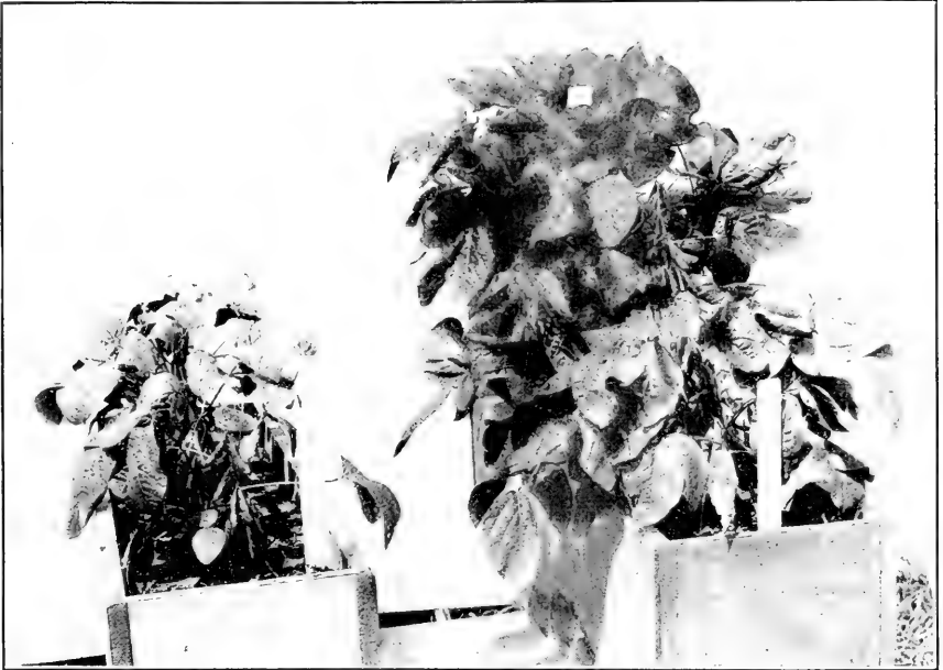
1. Biloxi soy bean. Plants in box on left exposed to light daily for 7 hours; those on right exposed 12 hours daily. While both lots blossomed and fruited promptly, the plants under the longer light exposure grew much larger than those under the shorter exposure. Photographed August 19.
