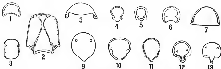
FIG. 12.—Opercula. Sketches showing the operculum in different genera of Cheilostomata.
