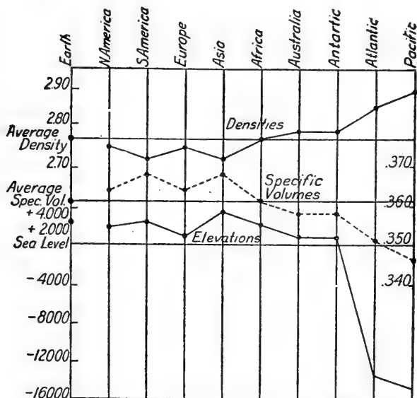
FIG. 3.—Elevations and densities of the continents.
