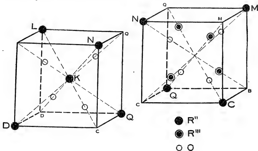
FIG. 26.—The spinel arrangement. The divalent metal atoms of a spinel occupy all of the positions of Fig. 24. The arrangement of the other atoms is here shown for the two typical divisions of this unit. Each divalent metal atom ( R'' ) is equally distant from four atoms each trivalent metal atom ( R''' ) from six atoms; and each divalent oxygen atom ( O ) from four atoms.
