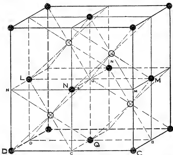
FIG. 24.—The zinc sulphide arrangement. In this arrangement each white atom is distant from four black atoms and each black atom from four white ones.
