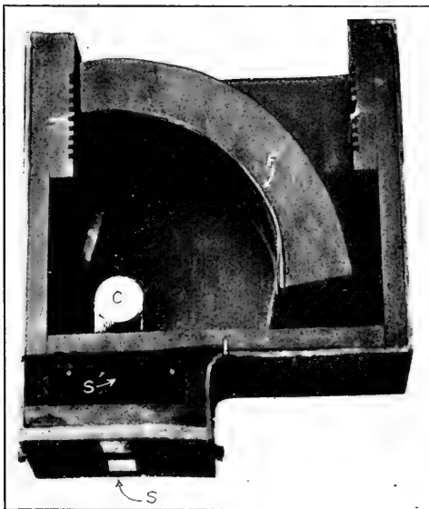
FIG. 13.—The front slit ( s ) is variable. The second one ( s' ) is fixed at a considerable width so that the beam of X rays striking the crystal mounted on the rotating table ( C ) is somewhat divergent. The photographic film is curved to the arc of a circle along F .
