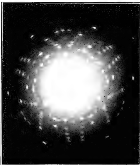
FIG. 7.—Calcite. Rhombohedral. X rays normal to the base (111).
