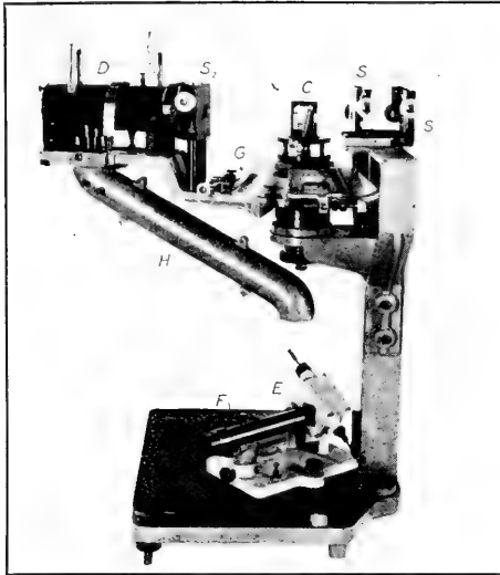
FIG. 12.—An X-ray spectrometer. G is a divided circle upon which the positions of the crystal and ionization chamber may be read; F is a microscope and scale for following the gold leaf of the electroscope ( E ); H is an earthed shield for the wire connecting the chamber and the electroscope.
