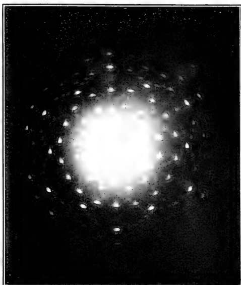
FIG. 6.—Carborundum twinned to give an hexagonal pattern. X rays normal to the (0001) face.
