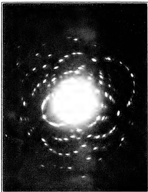
FIG. 8.—Calcite. Rhombohedral. X rays normal to the cleavage (100) face.
