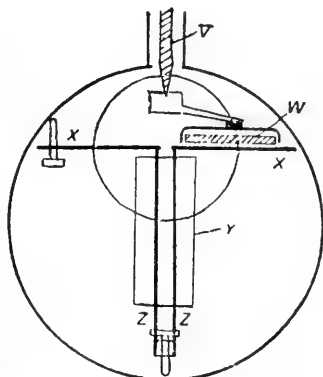
FIG. 4.—The camera.
