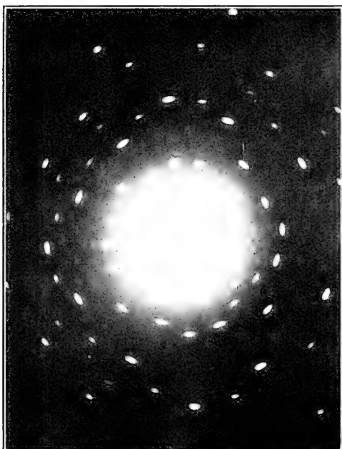
FIG. 9.—Magnesium oxide. Cubic. X rays normal to the cube (100) face.
