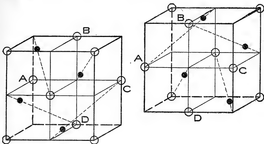
FIG. 25.—The pyrite arrangement. The black sulphur atoms are so spaced along the diagonals of these little cubes that each iron atom has six and each sulphur atom four equally near atoms.
