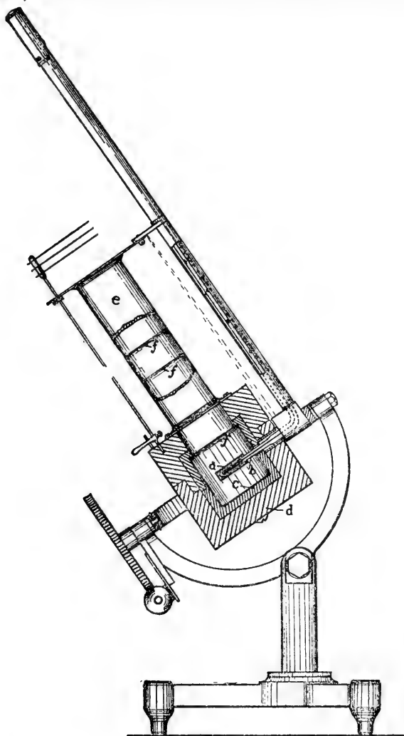
FIG. 1.—Abbot silver disk pyrheliometer.
