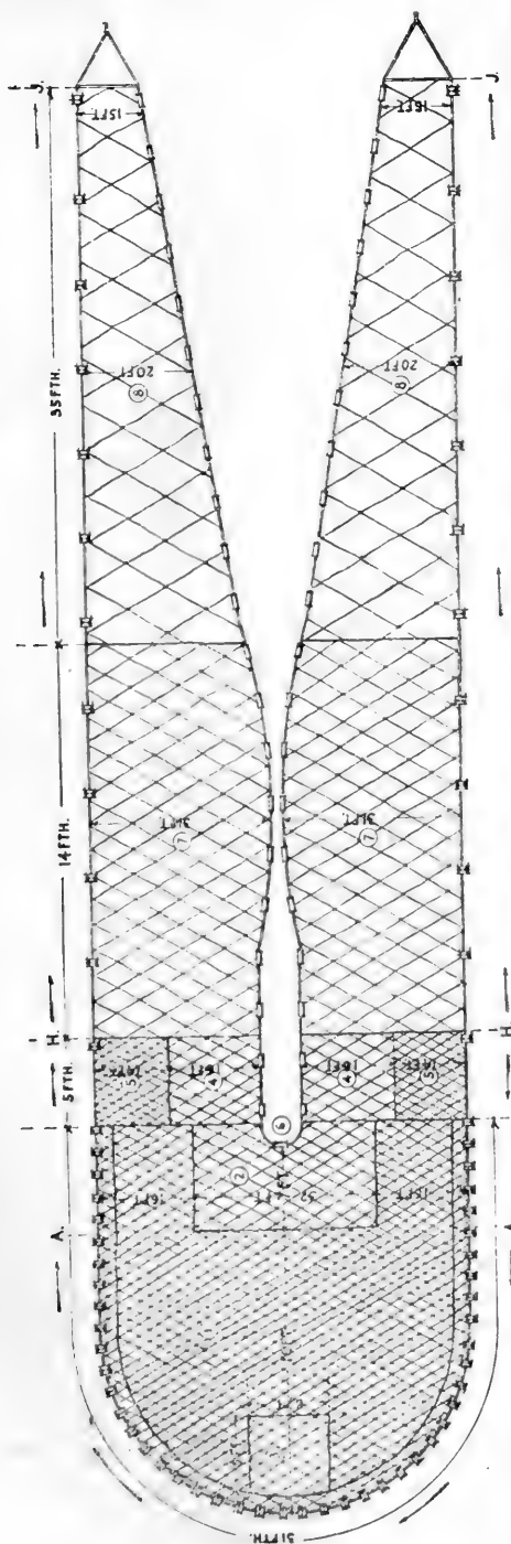
Fig. 3.—Lampara net. Section 1, 28-6 thread, \frac{1}{2} -inch mesh; 2, Mendocino or key of net 6-ply, 3-inch mesh; 3, heavy netting, 6-ply, 1-inch mesh, 8 by 8 feet; 4, 6-ply, 3-inch mesh; 5, part of bag of 28-6 thread, \frac{1}{2} -inch mesh; 6, horseshoe, where wings divide; 7, wing-section of 2-inch mesh; 8, wing-section of 8-inch mesh; 9, strip of netting 10 inches wide, 16-ply, 1-inch mesh of heavy mesh, to hold bag to cork line and withstand wear and tear; H-H, cork line of \frac{3}{8} -inch diameter lamp rope, 500 corks in pairs, 6-inch interspace between pairs; I-I, wing cork lines, 500 corks in pairs on each wing, interspaces about 3 feet.
