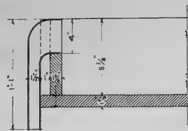
LONGITUDINAL SECTION THROUGH SUPPLY TROUGH
