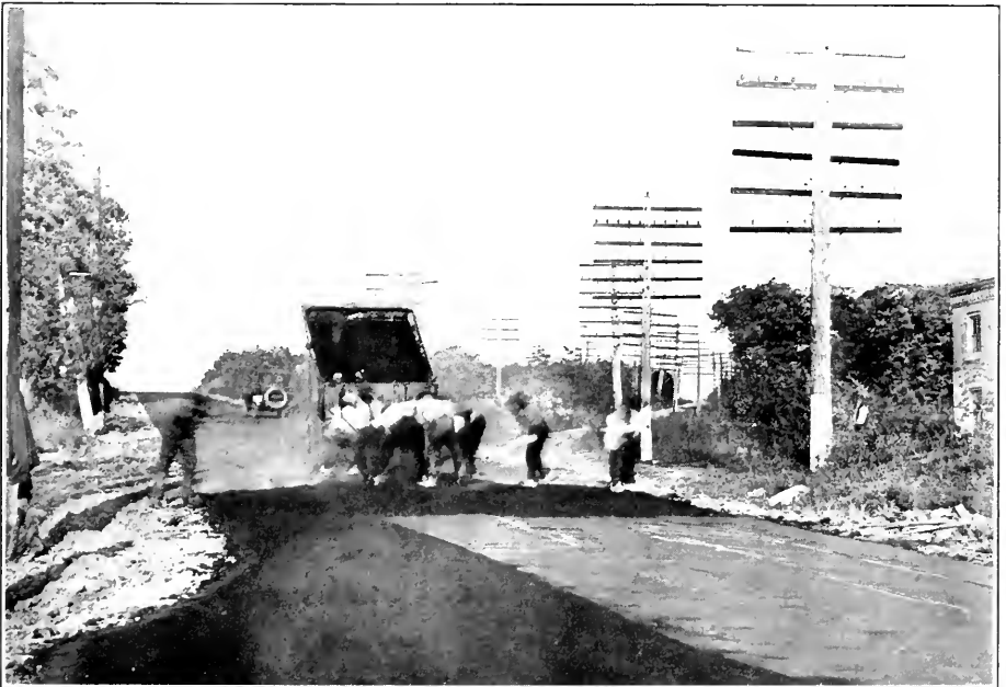
VIEW SHOWING ASPHALT BEING DELIVERED AND SPREAD ON BALTIMORE AND WASHINGTON BOULEVARD, IN BALTIMORE COUNTY
