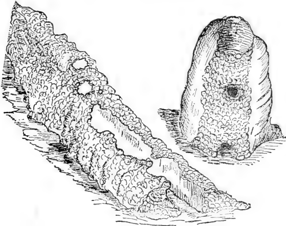
Fig. 30—ANT ENGINEERING
