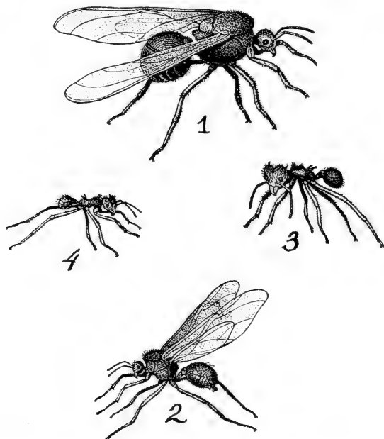
Fig. 49—CUTTING ANTS
