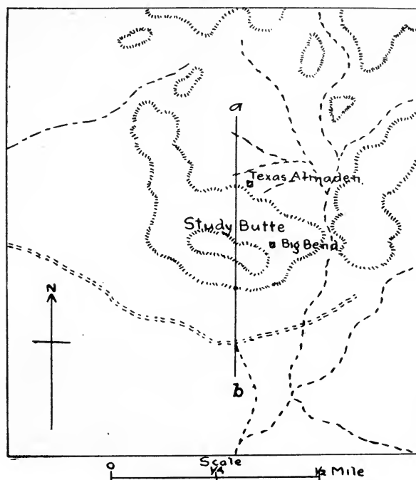
Fig. 6. Sketch map of Study Butte showing the position of the section in Fig. 7.
