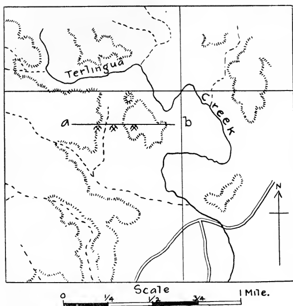
Fig. 10. Map of Section 248, and parts of sections 247, 230, and 299, Block G-4, west of the Chisos Mountains, Brewster County, showing location of section a-b, in Fig. 11.
