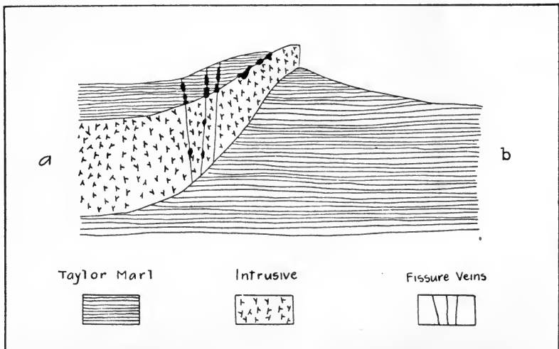
Fig. 7. Section of Study Butte extending from north to south along the line indicated in Fig. 6. Known occurrences of cinnabar-bearing rock roughly indicated by solid black.
