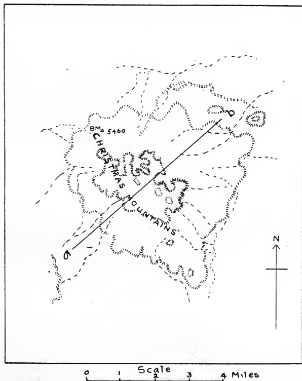
Fig. 8. Map of Christmas Mountain showing approximate position of section in Fig. 9.
