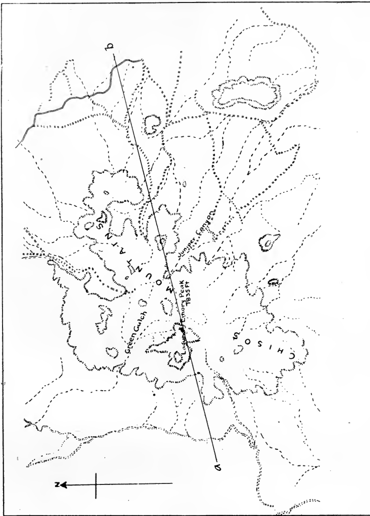
Fig. 12. Sketch map of the Chisos Mountains showing position of the section in Fig. 13.
