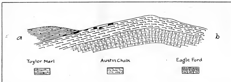
Fig. 11. Diagrammatic section along the line a-b in Fig. 10. Known occurrences of cinnabar are indicated by solid black.
