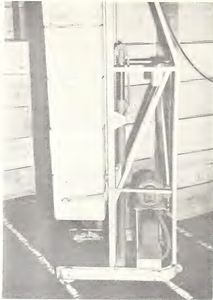
Figure 2.--Mechanical high-piler. With this equipment one worker, alone, can place 5 crates at a time in high storage position.
