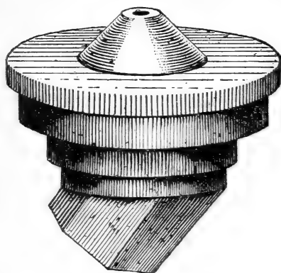
FIG. 5.—An excellent type of angle spray nozzle. The liquid enters the eddy chamber through an opening at the side and also through a hole in the center, directly under the orifice of the conical tip. By this construction a long, slender, solid cone of driving spray is produced.
