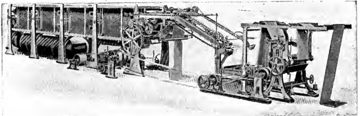
• FIG. 107.—Tentering and Drying Machine.
