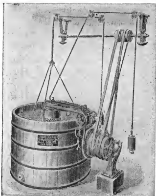
FIG. 126.—Dyeing Machine for Loose Stock. (Esser.)
