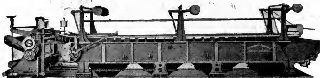
FIG. 56.—Wool Washer. (C. G. Sargent's Sons.)
