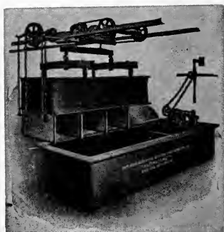
FIG. 165.—Circulating Dyeing Machine for Hosiery. (Philadelphia Dyeing Machine Co.)
