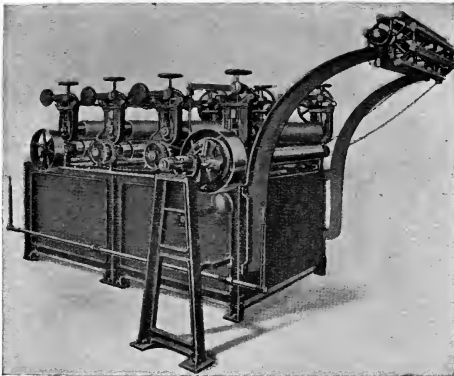
FIG. 68.—Open Washer for Piece-Goods. (Textile-Finishing Machinery Co.)
