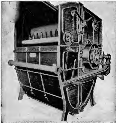
FIG. 72.—Cloth Washer. (Rodney Hunt Machine Co.)
