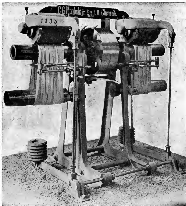
FIG. 29.—Yarn Glazing and Softening Machine.
