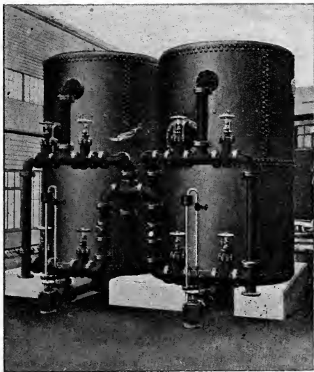
FIG. 92.—Water Softener. (Permutit System).
