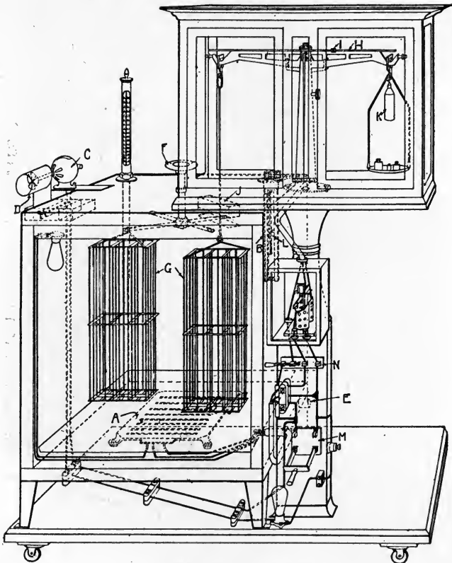
FIG. 46.—Emerson Textile Conditioning Oven.
