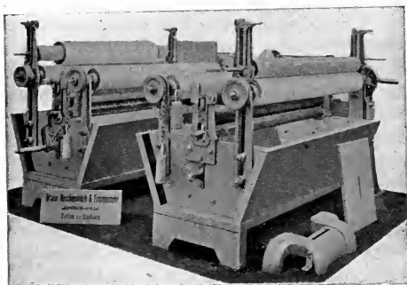
FIG. 183.—Jiggers for Mordanting and Dyeing. (Zittauer.)
