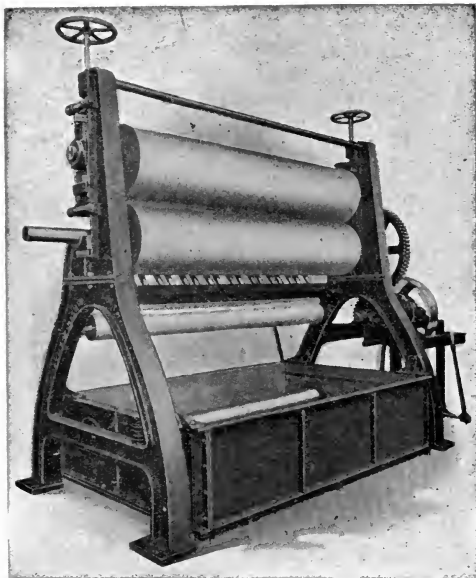
FIG. 101.—Bleach House Washer. (Textile-Finishing Machinery Co.)
