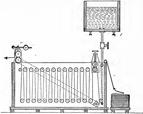
FIG. 212.—Dye Box for Continuous Dyeing Sulphur Colors.
