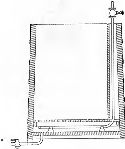
FIG. 18.—Round Wooden Dyevat, Vertical Section.
