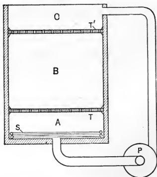
FIG. 20.—Showing General Principle of Pack System of Dyeing.
