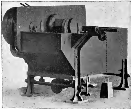
FIG. 243.—Yarn Impregnating and Wringing Machine. (Haubold).
