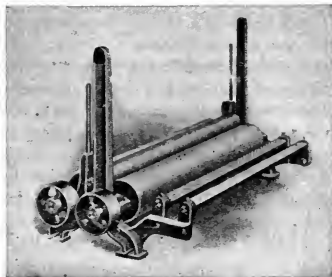
FIG. 258.—Rolling Machine. (Curtis & Marble.)
