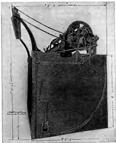
FIG. 117.—Roll Machine for Bleaching Knitgoods.
