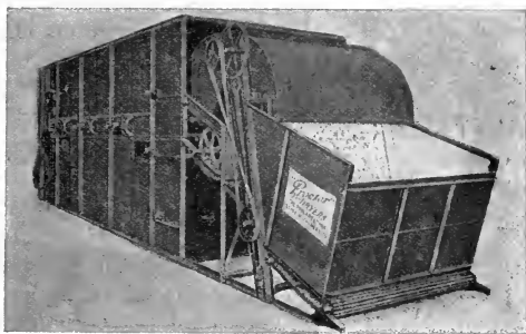
FIG. 133.—Automatic Dryer for Cotton, Wool, Raw Stock, etc. (Philadelphia Textile Machinery Co.)
