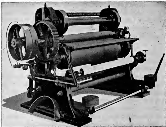
FIG. 296.—Gaufring and Embossing Machine.
