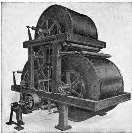
Fig. 256. —Three-Cylinder Back Drying Machine. (Textile-Finishing Machinery Co.)
