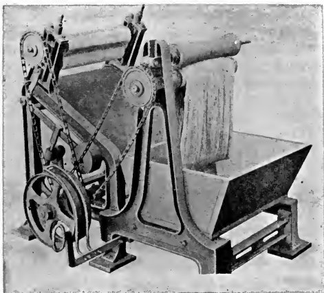
FIG. 299.—Sizing Machine for Skein Yarn.
