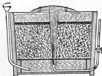
FIG. 21.—The Dreze Dyeing Machine. (Showing Pack System.)
