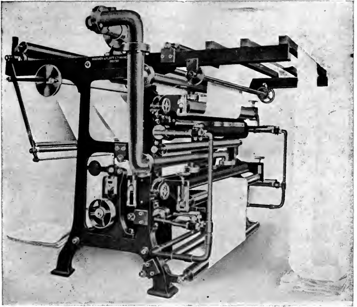
FIG. 95.—Two-Burner Gas Singeing Machine. (Mather & Platt).
