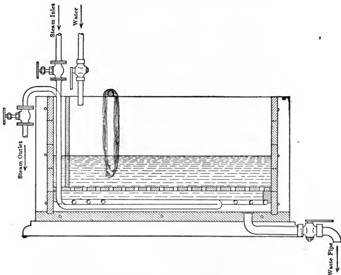
FIG. 15.—Dyevat for Yarn. (Indirect Steam.)
