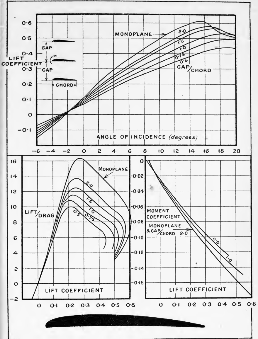
FIG. 78.—Variation of triplane gap.
