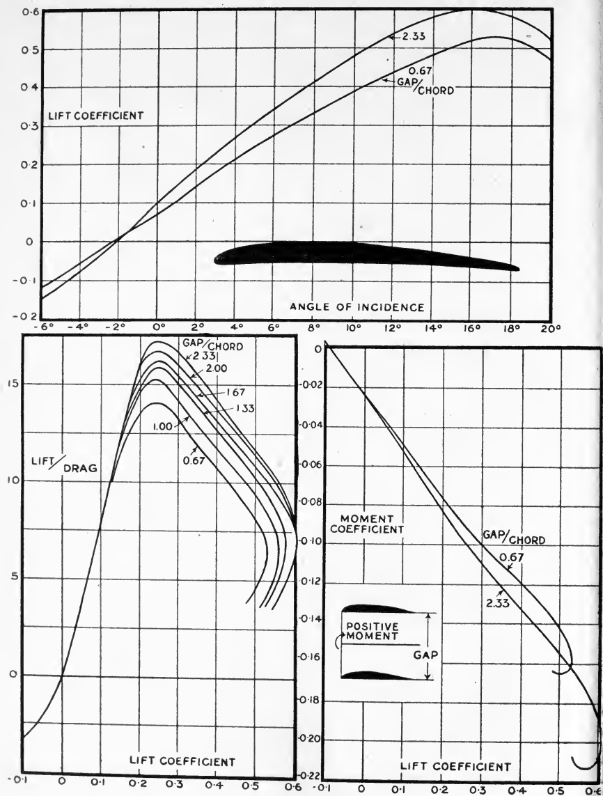
FIG. 74.—Variation of biplane gap.
