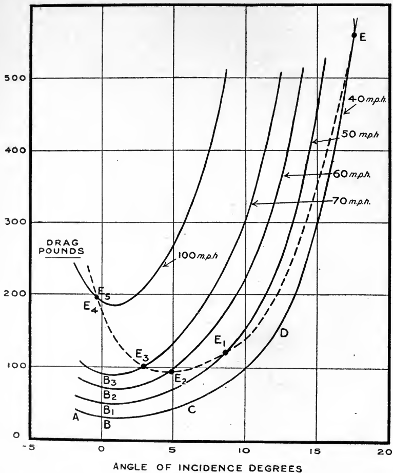
FIG. 13.—Wing drag and speed.
