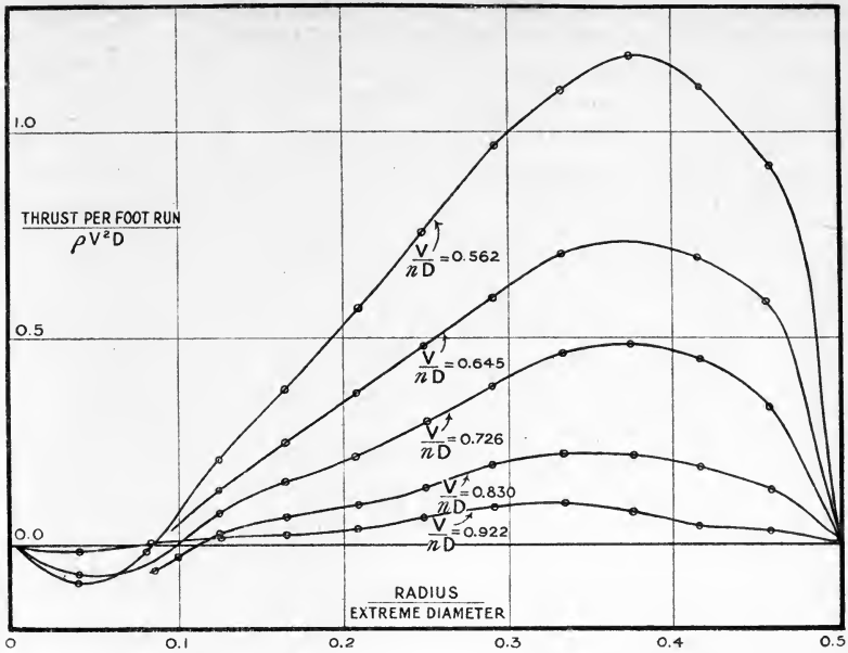
FIG. 144.—Thrust variation along an airscrew blade (experimental).
