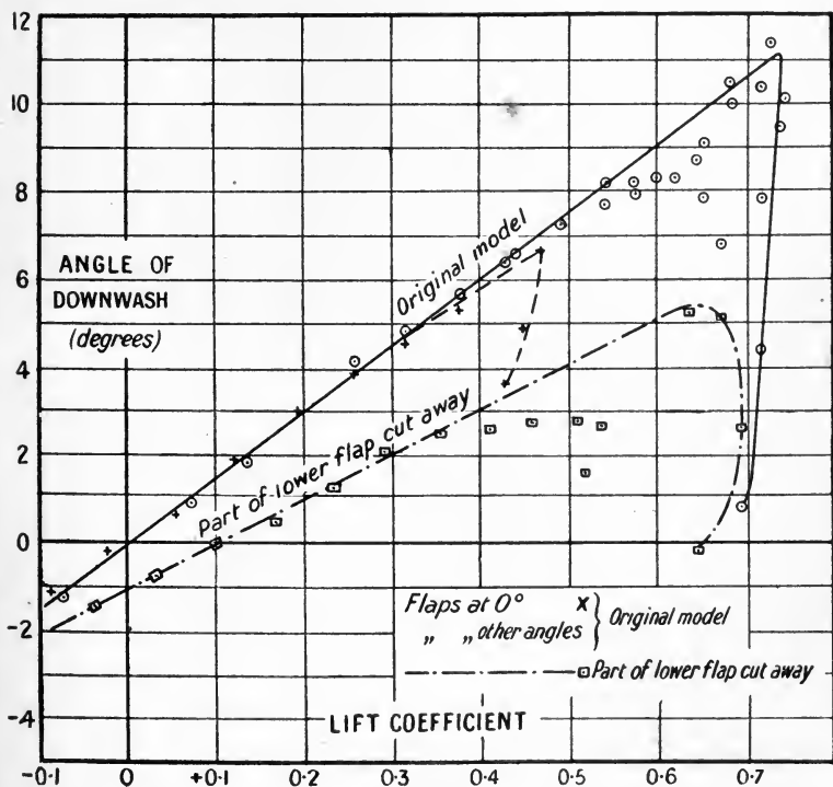
FIG. 98.—Downwash behind wings of variable section.
