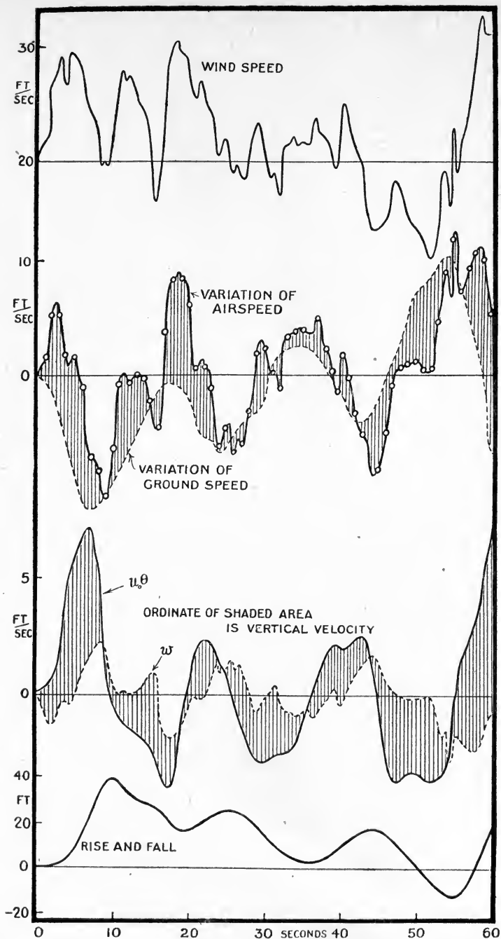
FIG. 252.—Uncontrolled flight in a natural wind (Aeroplane stable.)
