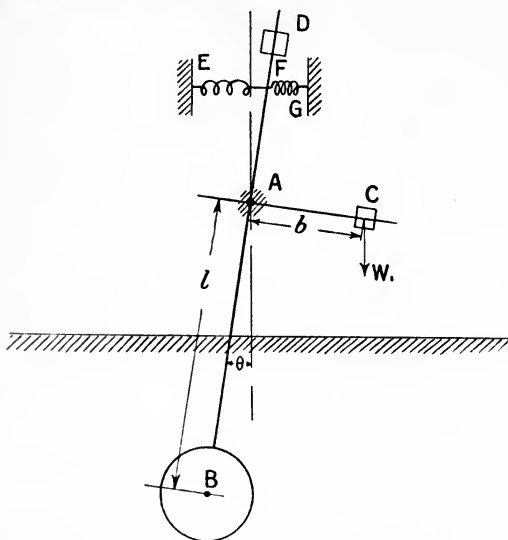
FIG. 62.—Forces due to acceleration of fluid motion.
