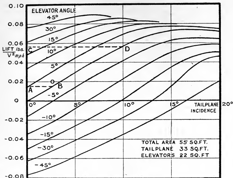
Fig. 33.—Lift of tail plane and elevator for different settings.
