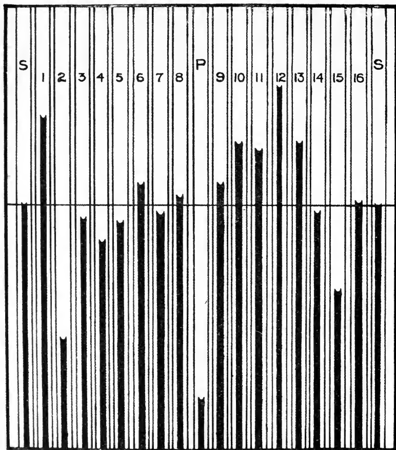
FIG. 48.—Photo-manometer record.
