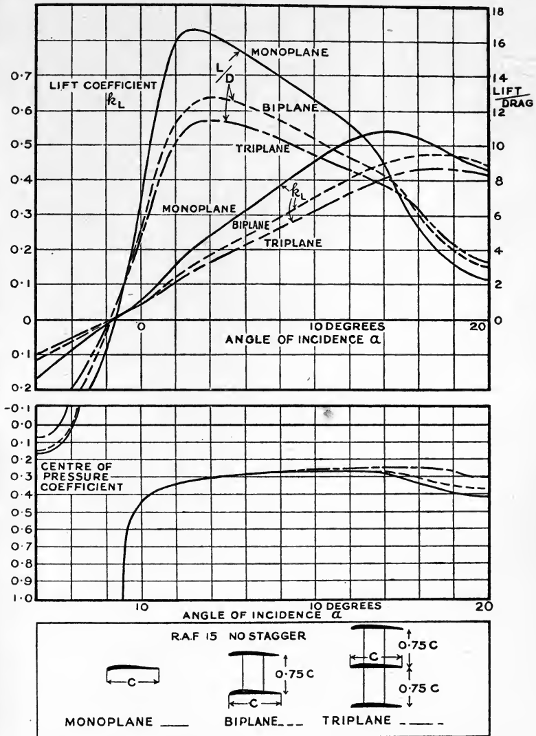
Fig. 73.—Biplane and triplane effects.
