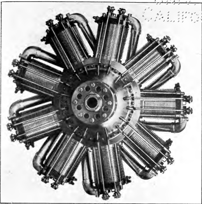
FIG. 5 (a).—Rotary engine.
