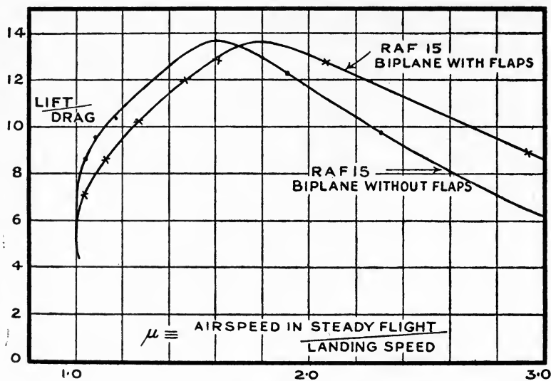
Fig. 77.—Comparison between fixed and variable section wings.
