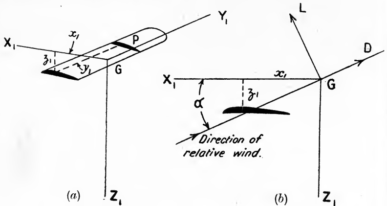
[ FIG. 142.—Aerofoil element theory.
