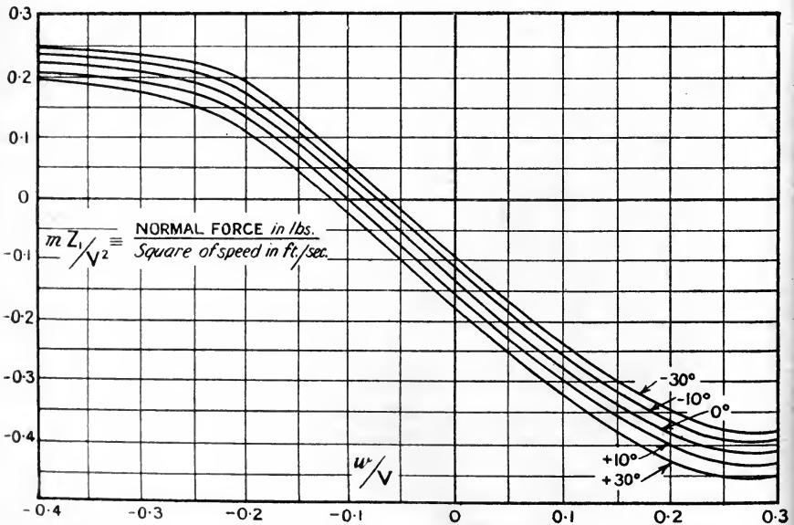
FIG. 131.—Normal force on an aeroplane due to inclination to the relative wind.
