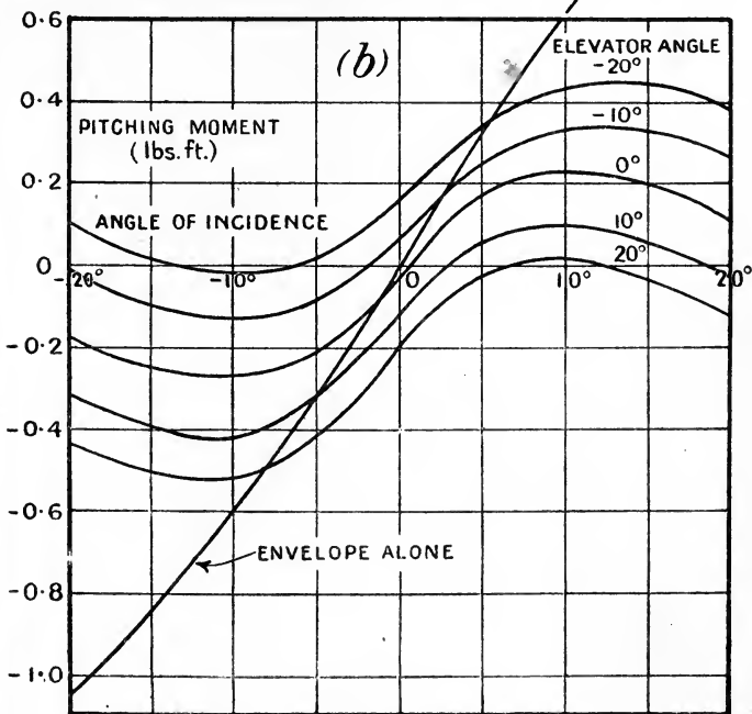
FIG. 104.—Forces and moments on a model of a rigid airship.
