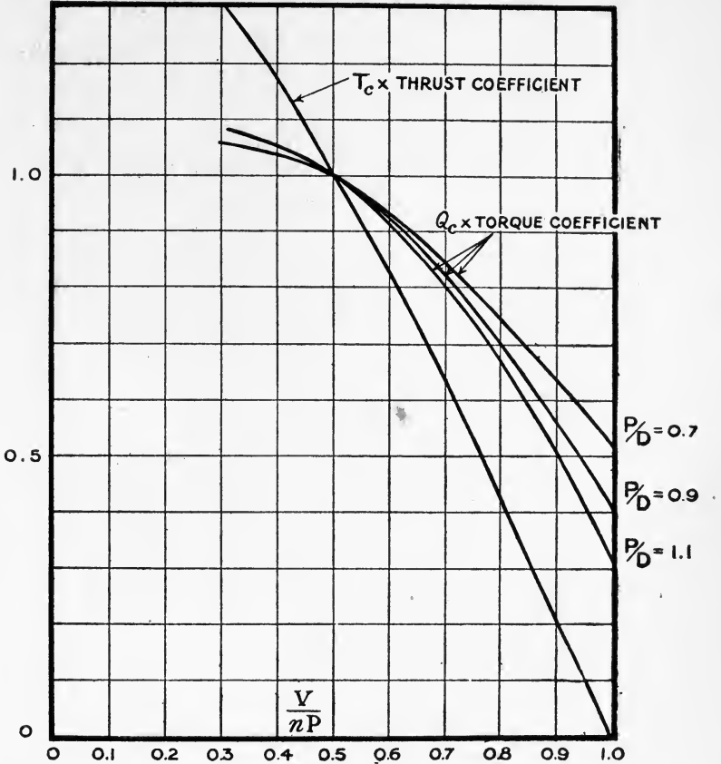
FIG. 159.—Standard airscrew characteristics.
