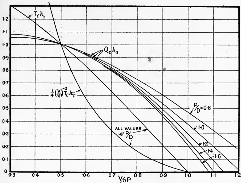
FIG. 218.—Standard airscrew curves used in the analysis of aeroplane performance.
