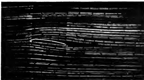
FIG. 179.—Viscous flow round wing section (free fluid).
