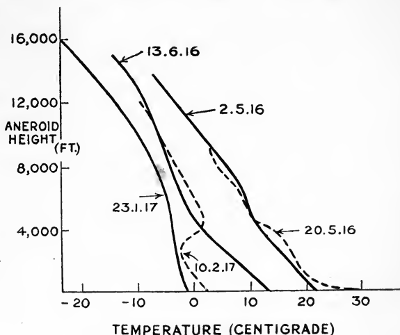
Fig. 201.—Atmospheric changes of temperature.
