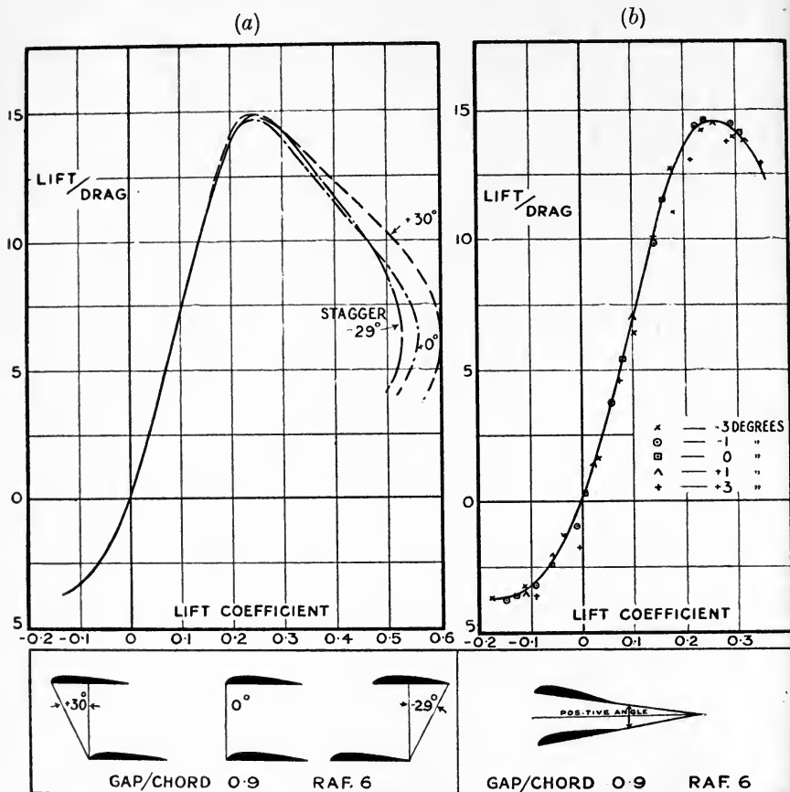
Fig. 75.—Variation of biplane stagger.
