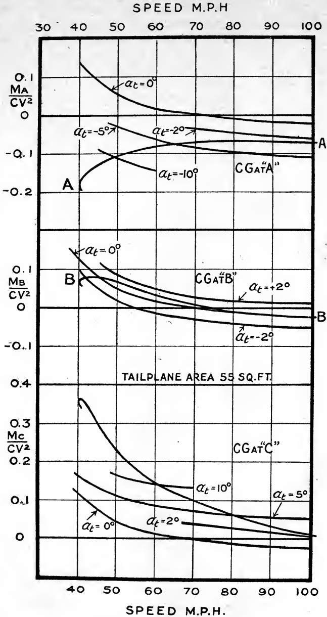
FIG. 28.—Longitudinal balance.
