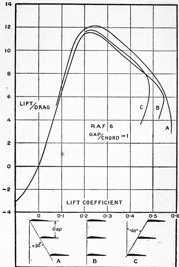
FIG. 79.—Variation of triplane stagger.
