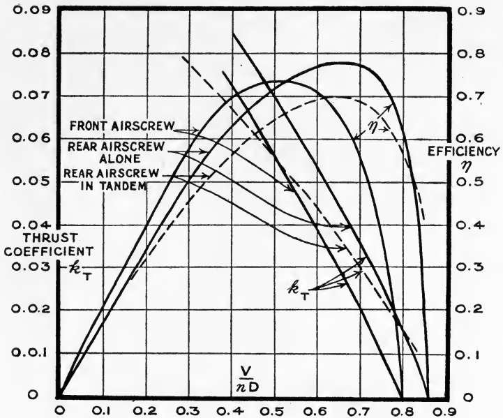
FIG. 155.—Tandem airscrews.
