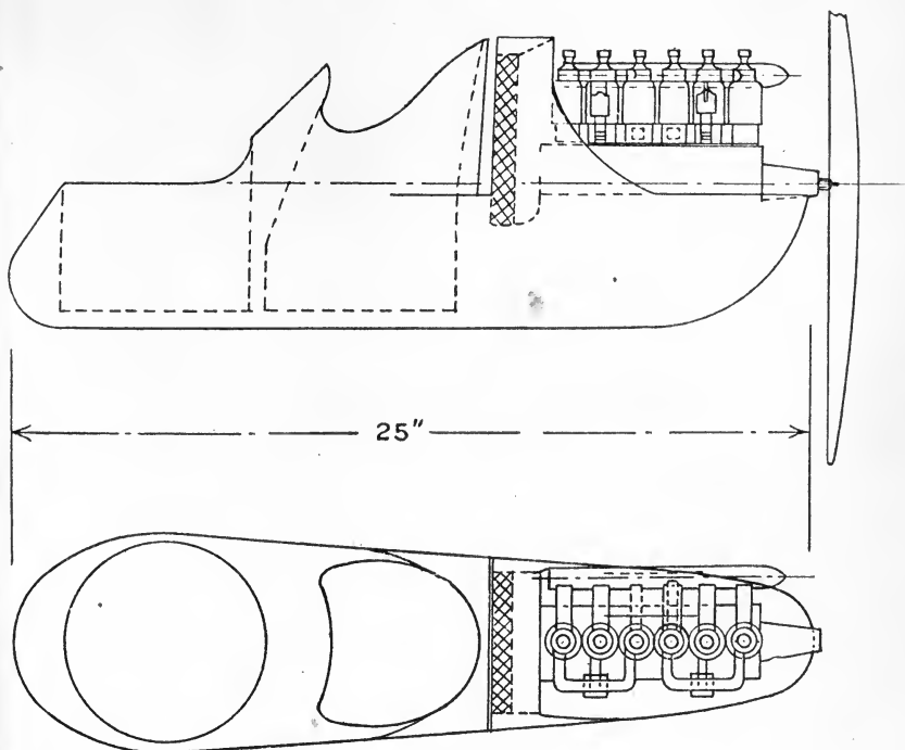
FIG. 90.—Pusher body.
