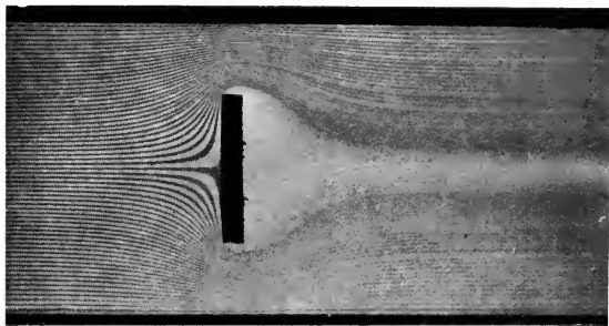
FIG. 177.—Viscous flow round section of flat plate (Hele-Shaw). High speed.
