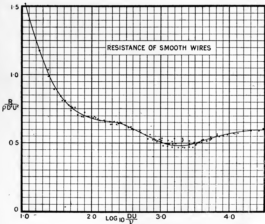
FIG. 193.—Application of the laws of similarity to the resistance of cylinders.
