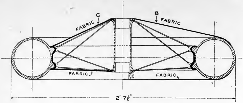
FIG. 91.—Aeroplane landing wheel.
