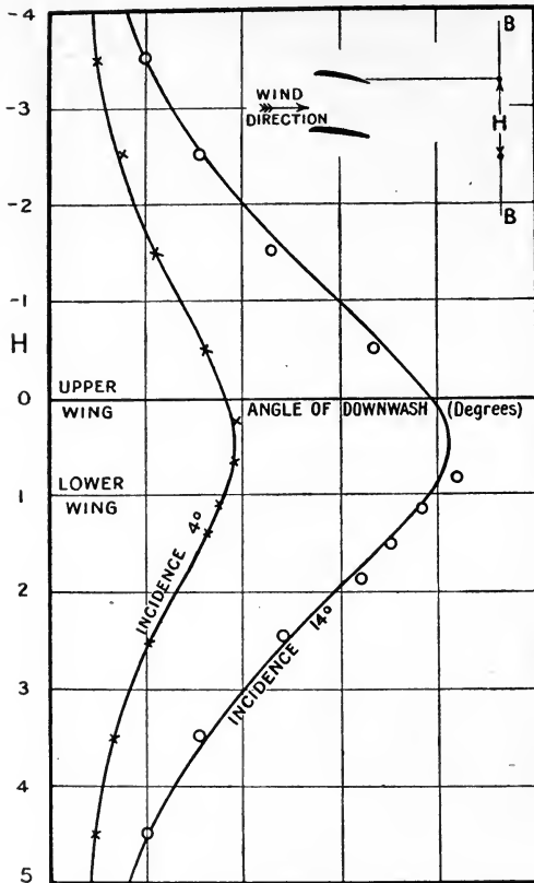
FIG. 97.—Vertical distribution of downwash.
