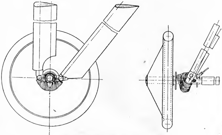
FIG. 93.—Model undercarriage as tested.
