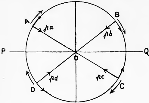
FIG. 185.—Cyclic flow round cylinder.
