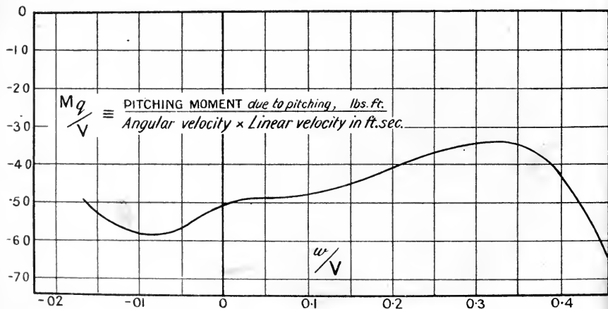
FIG. 134.—Pitching moment due to pitching of an aeroplane.
