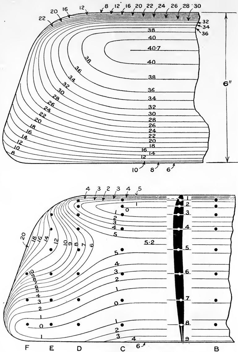
FIG. 80.—Model for pressure distribution on a wing.
