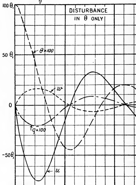
FIG. 247.—The effect of simple longitudinal disturbances. (Aeroplane stable.)
