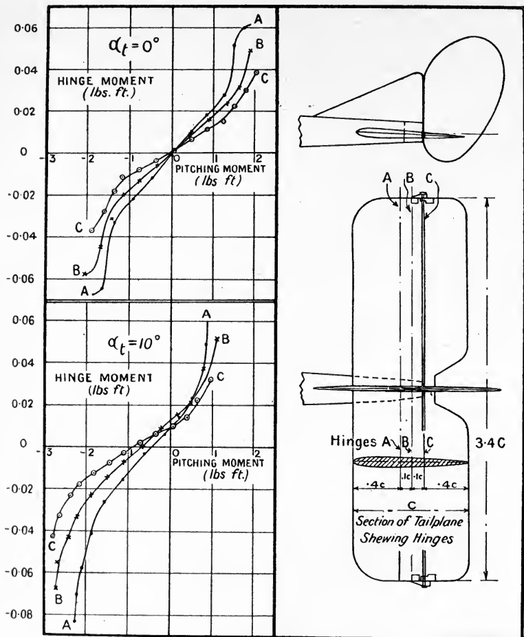
Fig. 99.—Variation of elevator area.
