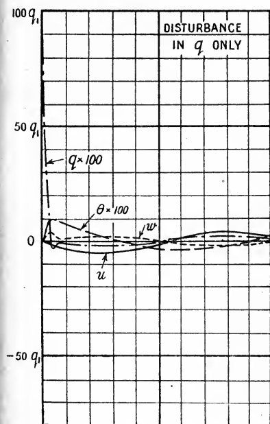
FIG. 247.—The effect of simple longitudinal disturbances. (Aeroplane stable.)
