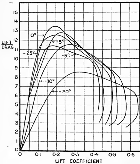
FIG. 76.—Biplane with wing flaps.
