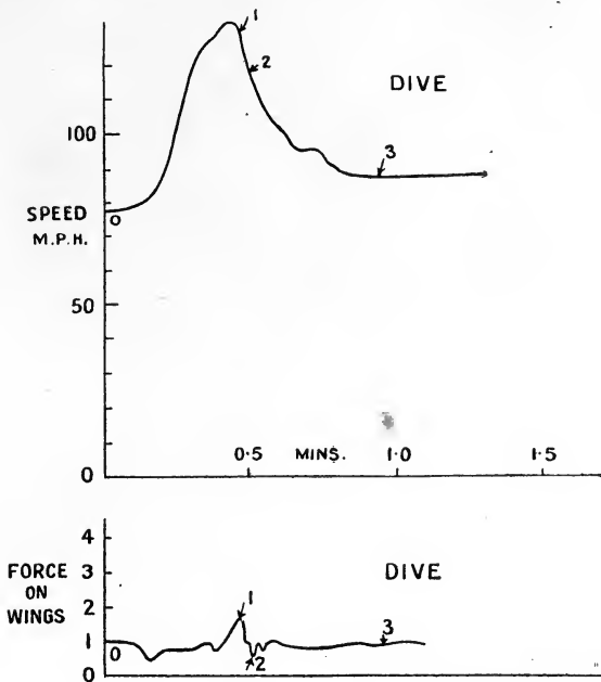
FIG. 125.—Speed and force on wings during a dive.
