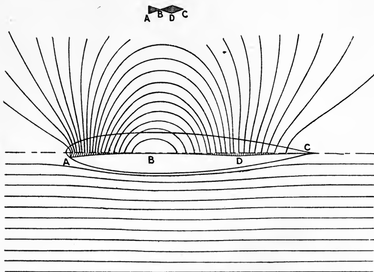
FIG. 183.—Calculated flow of inviscid fluid round an airship envelope.
