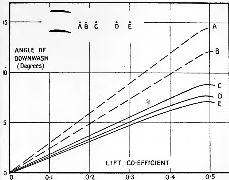
FIG. 96.—Downwash and lift coefficient.
