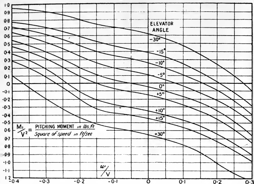
FIG. 133.—Pitching moment due to inclination of an aeroplane to the relative wind.
