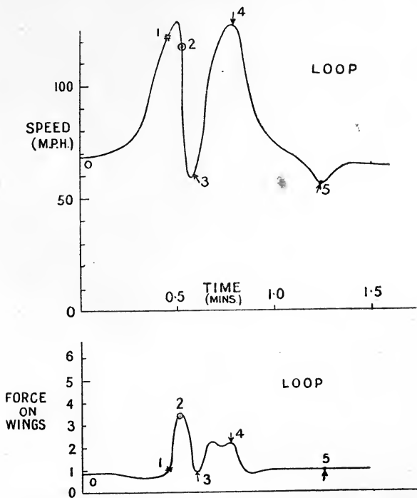
FIG. 123.—Speed and force on wings during a loop (observed).
