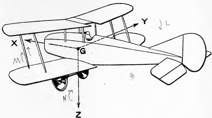
FIG. 106.—Standard axes.
