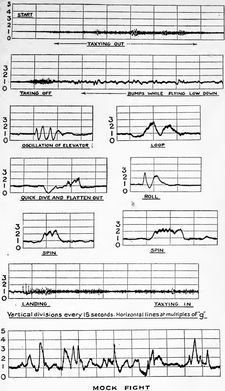
FIG. 45.—Accelerometer records.
