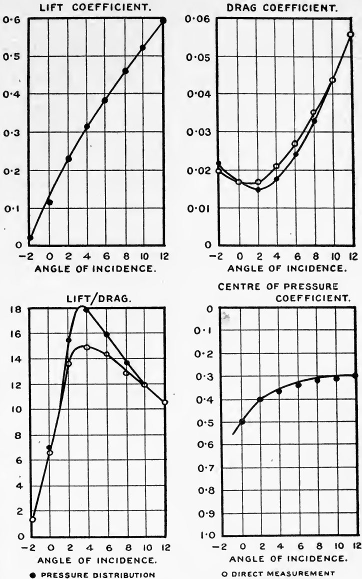
Fig. 85.—Comparison of forces and pressure integrals.
