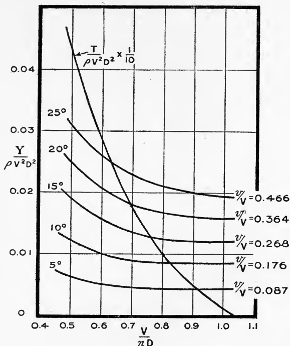
FIG. 162.—Lateral force on inclined airscrew.
