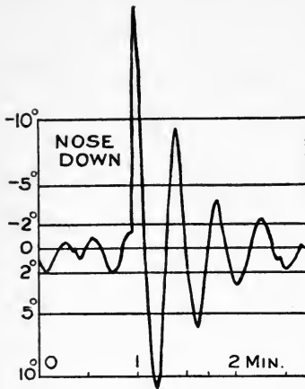
FIG. 49.—Stability record.
