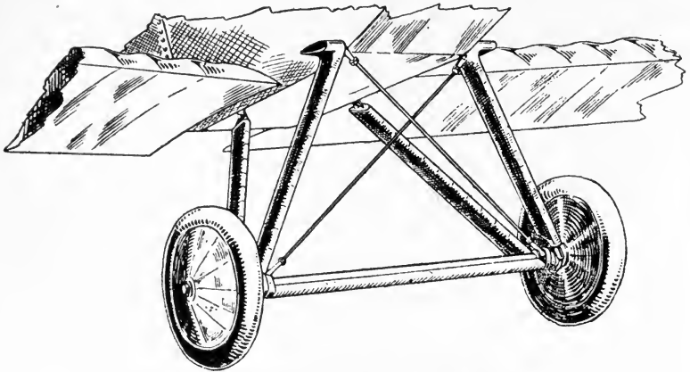
FIG. 92.—Aeroplane undercarriage.
