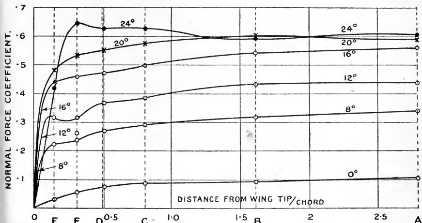
FIG. 84.—Force distribution along an aeroplane wing.
