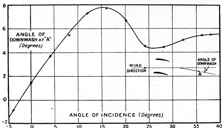
FIG. 95.—Downwash and angle of incidence.
