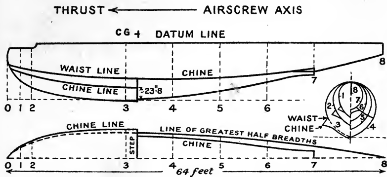
FIG. 35.—Flying boat hull.
