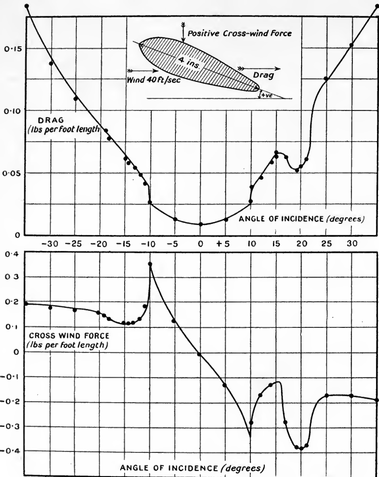
FIG. 87.—Forces on an inclined strut.
