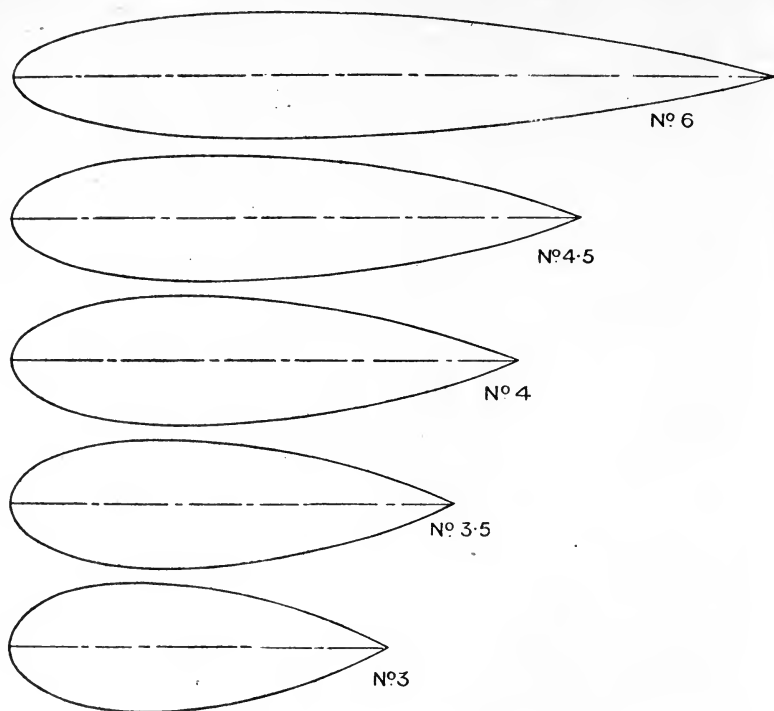
FIG. 100.—Airship envelope models.
