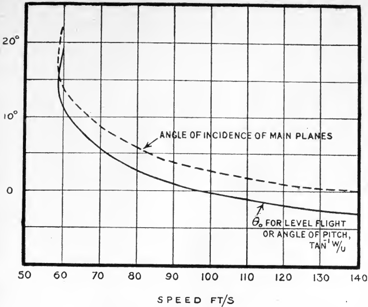
FIG. 238.—Angle of pitch and flight speed.
