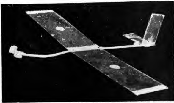
FIG. 232.—Model which develops an unstable phugoid oscillation. Large moment of inertia fore and aft with small restoring couple.
