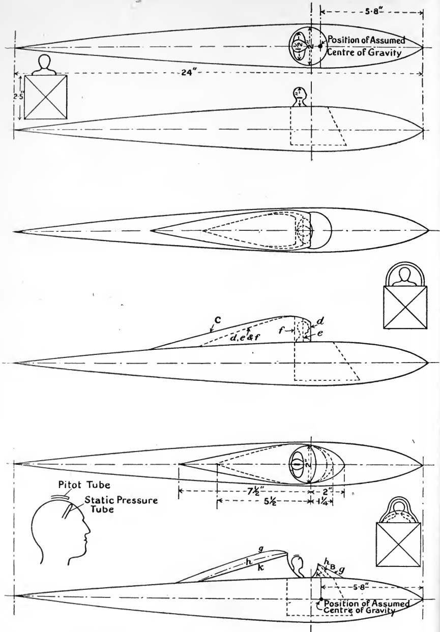
FIG. 88.—Model of aeroplane body and certain modifications.
