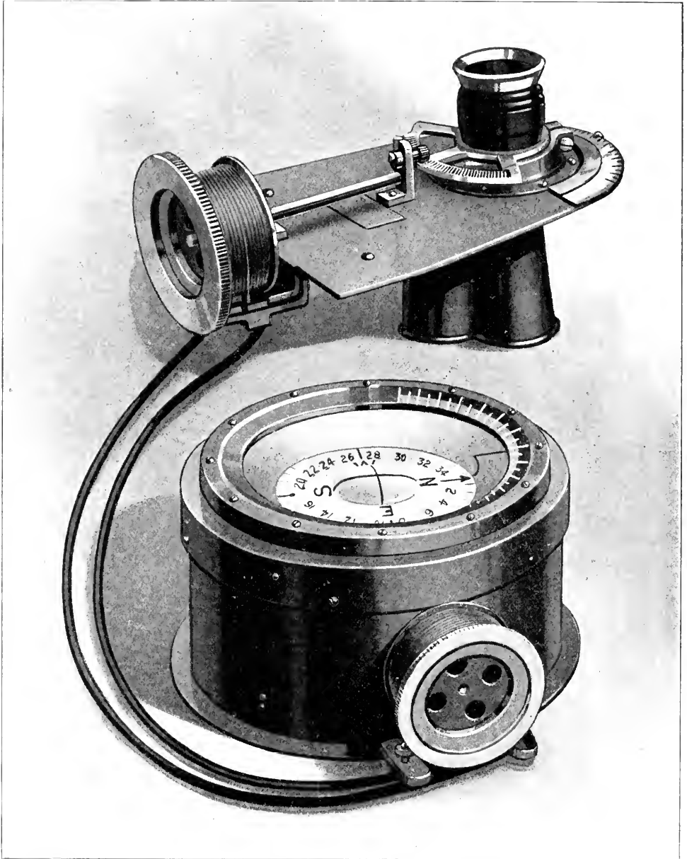
Fig. 63—Sperry Automatic Drift Set, consisting of a small revolving telescope which is connected to compass case in such a way that compass case with lubber line is automatically turned to compensate for side drift when sighting telescope is turned to line up cross-hairs with apparent motion of plane over ground
