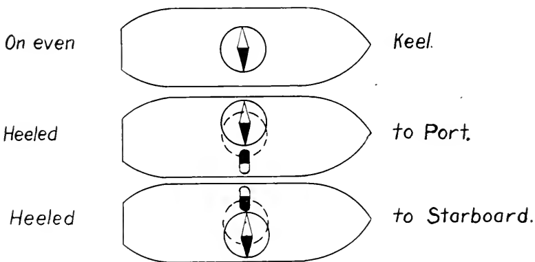
Fig. 51—Showing compass error due to heeling of ship when heeled north or south
