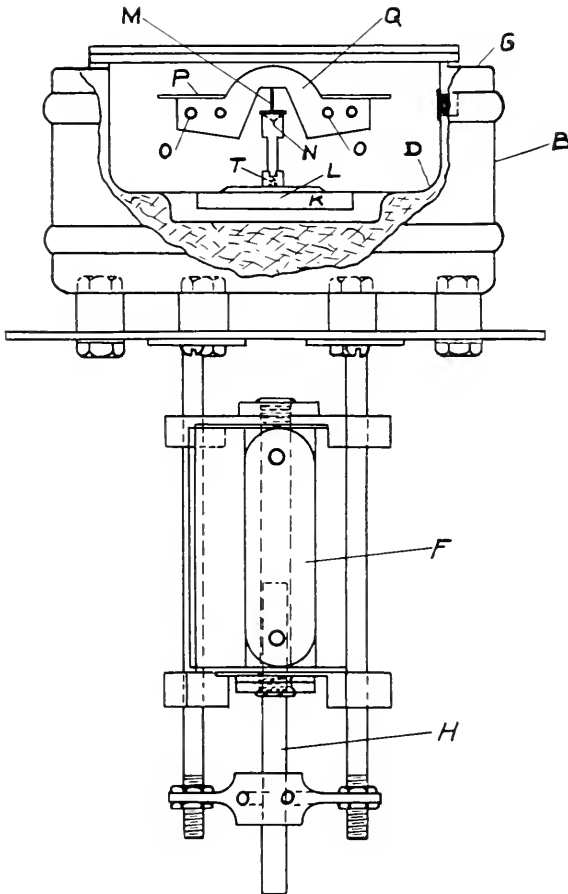
Fig. 46—Details of the Creagh Osborn airplane compass
