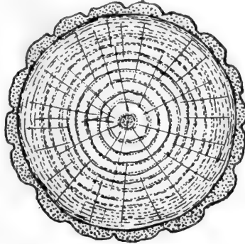
FIG. 73.—Sieve tissue.
