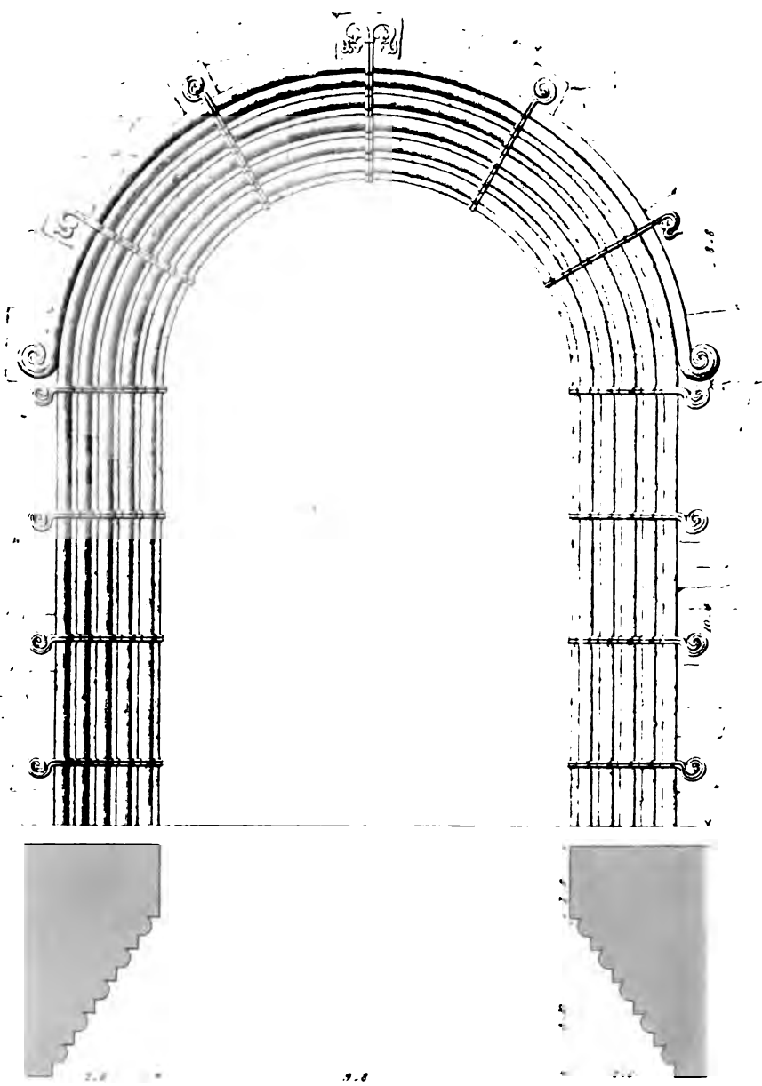
WEST DOORWAY OF NAVE. STRATA FLORIDA ABBEY. Scale 1/4 inch to 1 foot
