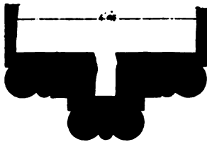
Strata Florida Abbey Section of Arches of Nave Arcade.
