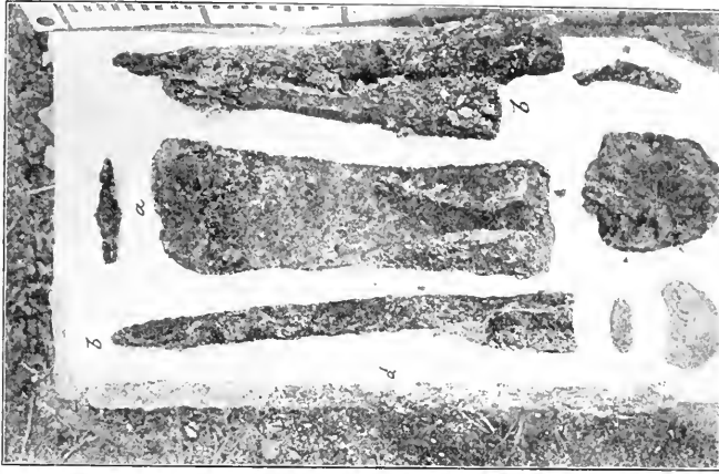
FIG. 76. PLOWSHARES FROM MEGIDDO (after Schumacher).
