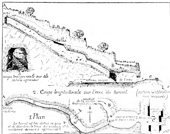
FIG. 63. PLAN OF UNDERGROUND TUNNEL AT GIBEON (after Abel).
