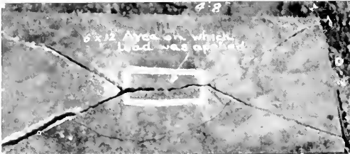
Portion of slab cast for Method E, 11', "x24"x4'-8", was bedded on concrete 2"x4" supports at sides of slab. The only reinforcing in the slab was 18-gauge stucco netting. The slab broke under the second application of a 2000 pound concentration on a central 6"x12" area.
