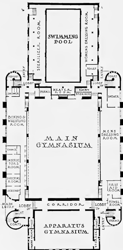
PLAN, STATE TEACHERS COLLEGE, SAN JOSE George B. McDougall, State Architect
