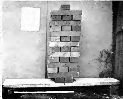
Slab No. 21. 1 1/2" x 12" (no reinforcing) Span 40", Central load 295#. Ult. L. = 321# M = 1/8" x 3210 + 300 (for slab wt.) = 3510# Modulus of Rupture = M = bd^2/6 = 1,120 psi Note that the specimens reported above were allowed to set and were cured without restraint (other than that provided by form friction and by the bars in specimen No. 23) Fractures of 21, 22, & 24 showed aggregate pulled apart on tension side of slabs; even small particles of hard gravel.
