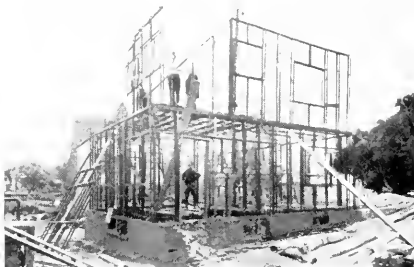
First floor steel frame in place and part of second floor frame work up
