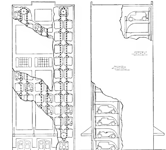
LEFT: CUT AWAY FRONT VIEW, SHOWING METHOD OF ATTACHING CRADLES TO ENDLESS CHAIN. RIGHT: SIDE VIEW SHOWING HOW CARS ARE CARRIED IN INDIVIDUAL CRADLES.
