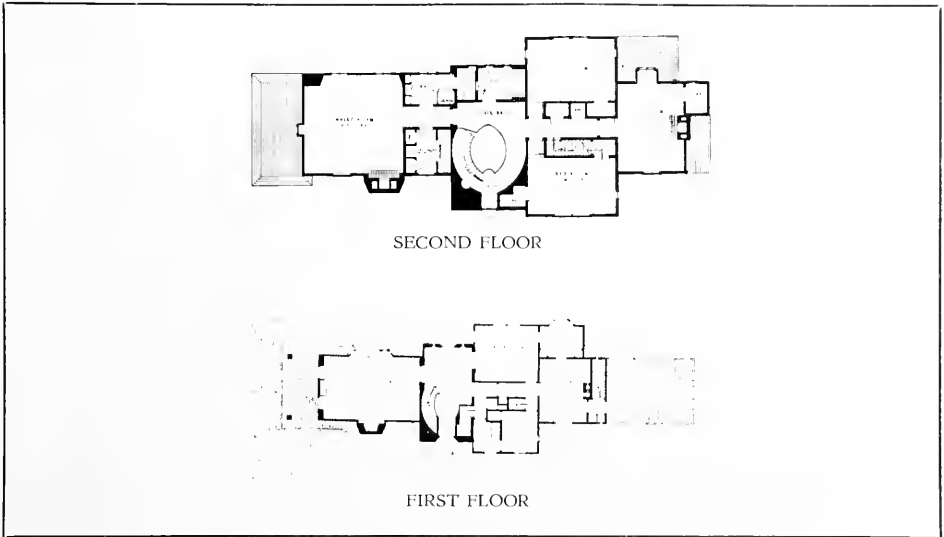
PLANS, RESIDENCE OF LELAND JAMES, PORTLAND, OREGON Harold W. Doty, Architect
