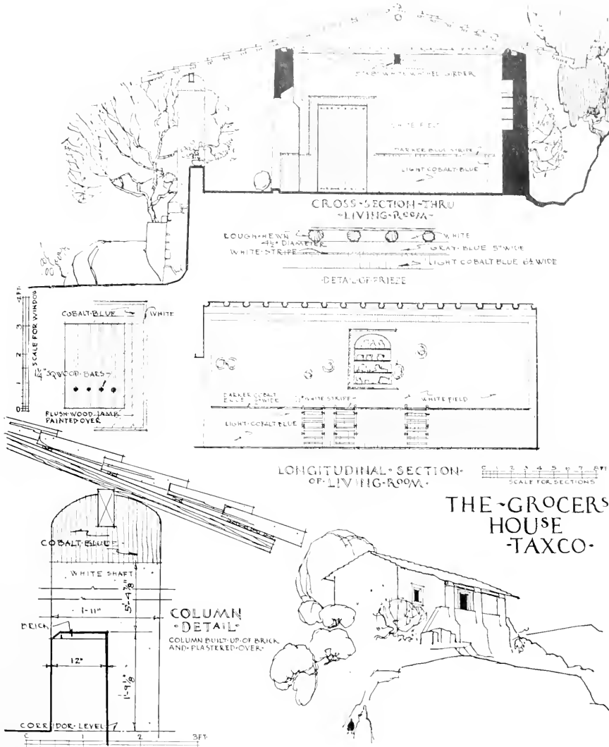
MEASURED DRAWINGS, THE GROCER'S HOUSE, TAXCO, STATE OF GUERRERO REPRODUCED BY SPECIAL PERMISSION FROM "MEXICAN HOUSES"
