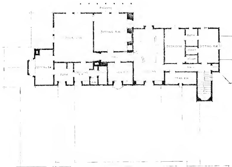
SECOND FLOOR PLAN 1" = 4'-0"
