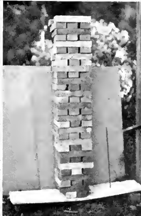
Slab No. 23; 1 1/2" x 12", reinforced with 2-1/2" dia. (1/2") Span 40", Central load, 630#. Ult. L. = 651# M = 1/8" x 6500 + 300 (for slab wt.) = 6800# f c = 3,400 psi; f s = 65,000 psi Failure due to slipping of bars (bond failure)
