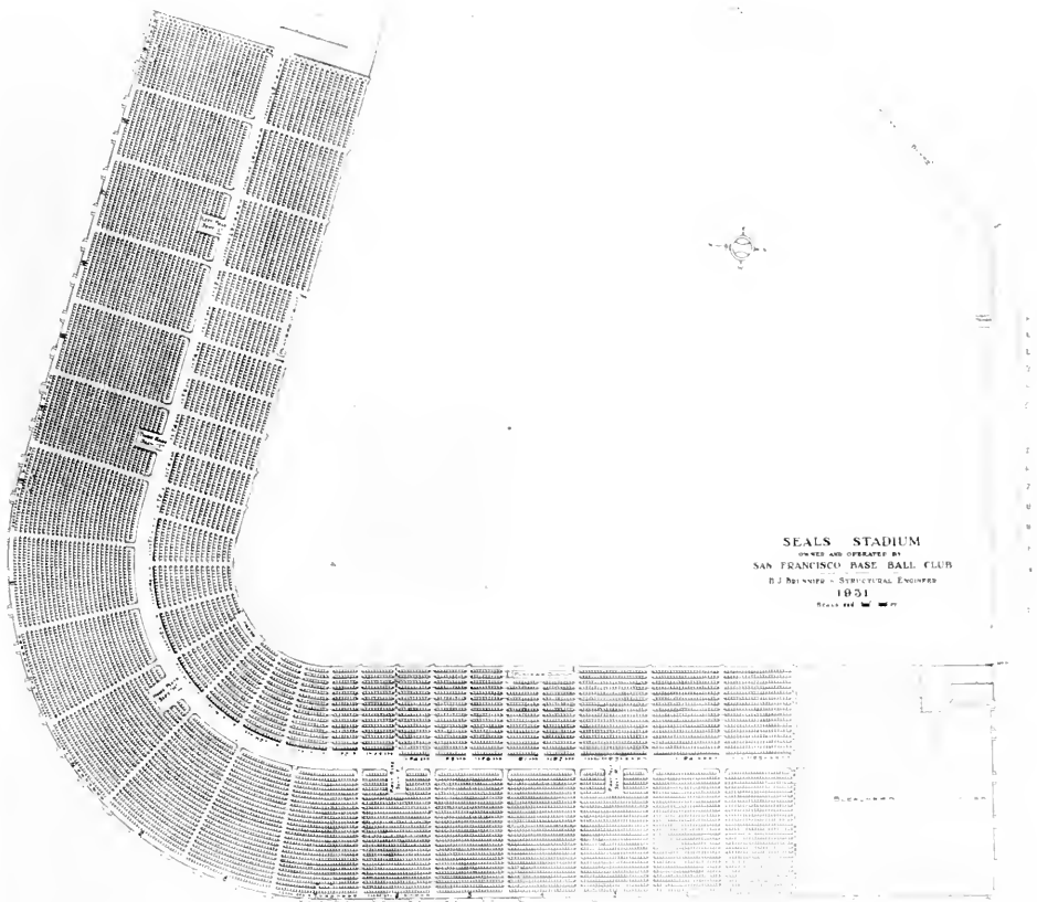
SEATING LAYOUT, SEALS' STADIUM, SAN FRANCISCO H. J. Brunnier, Structural Engineer
