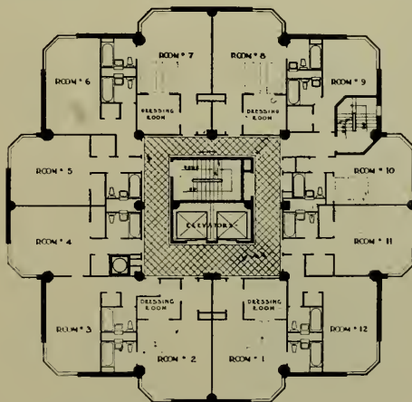
PLAN OF TOWER, EDMOND MEANY HOTEL, SEATTLE, WASHINGTON R. C. Reamer, Architect
