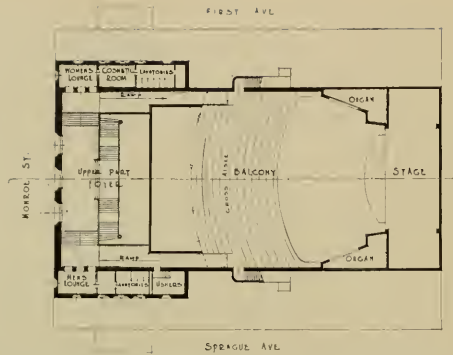
PLAN, FOX THEATER, SPOKANE WASHINGTON R. C. Reamer, Architect
