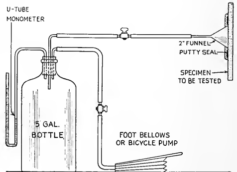
Fig. 2—Arrangement of apparatus for determining the porosity of acoustical plaster.
