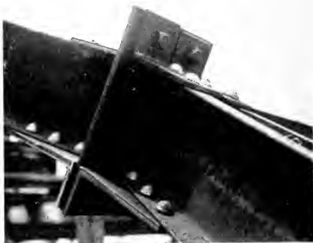
DETAIL OF STEEL LAMELLA ROOF, COCO COLA WAREHOUSE, LOS ANGELES
