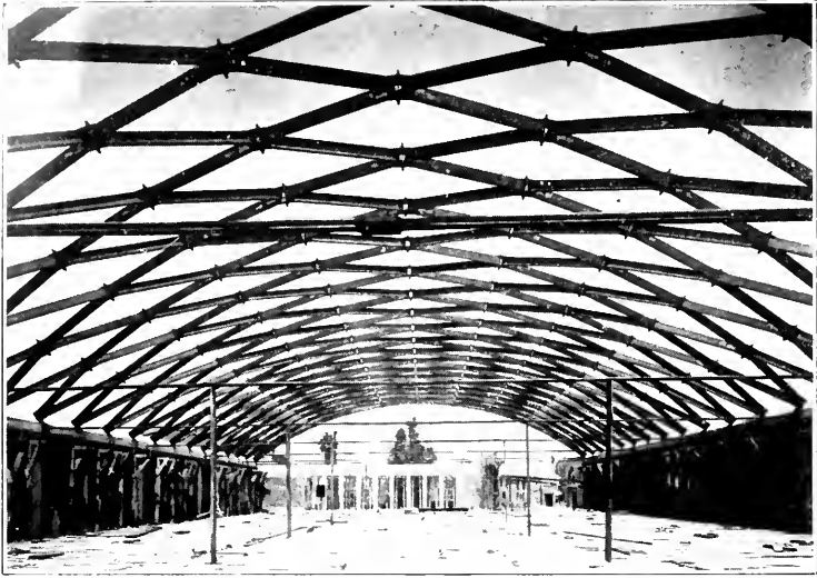
INTERIOR VIEW OF ROOF CONSTRUCTION, SHOWING STEEL TRUSSES BEFORE ENCASED IN CONCRETE
