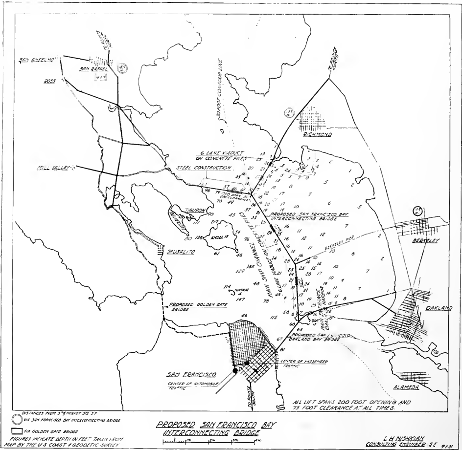
SUGGESTED COURSE OF PROPOSED SAN FRANCISCO BAY INTER-CONNECTING BRIDGE L. H. Nishkian, Consulting Engineer.
