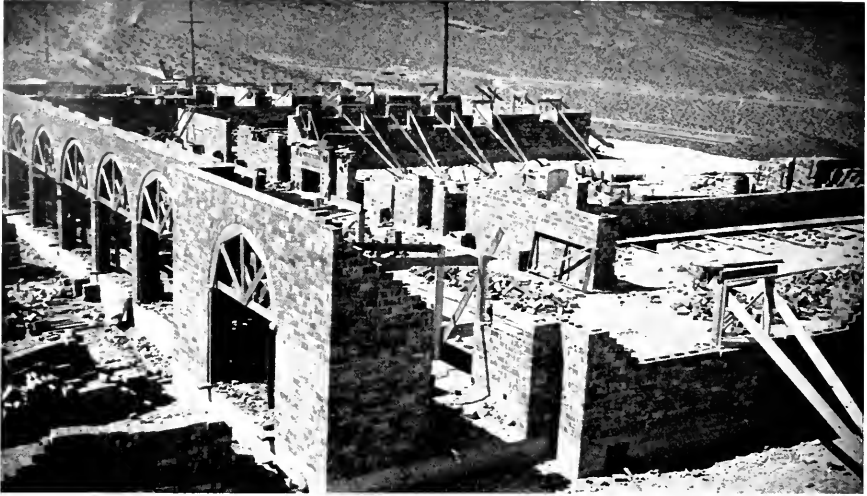
BOULDER CITY, NEVADA General view of a dormitory building under construction.
