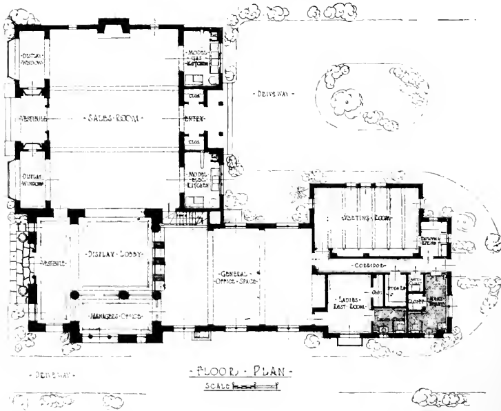
GROUND PLAN, BUILDING FOR COAST COUNTIES GAS & ELECTRIC COMPANY, WATSONVILLE Albert F. Roller, Architect
