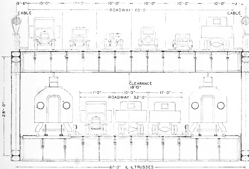
CROSS SECTION WEST BAY SPAN, SAN FRANCISCO-OAKLAND BAY BRIDGE Department of Public Works, State of California
