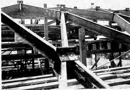
BRACKETS RIVETED TO ENDS OF STEEL CHANNEL LAMELLAS AND BOLTED TOGETHER THROUGH STEEL PLATES
