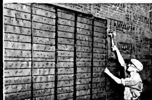
Ribbed STEELTEX Lath for plaster and STEELTEX Channels form a practical and modern method of constructing school partitions.
