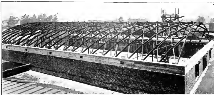
STEEL LAMELLA ROOF, COCO COLA PLANT, LOS ANGELES. THIS ROOF HAS A 70-FOOT SPAN
