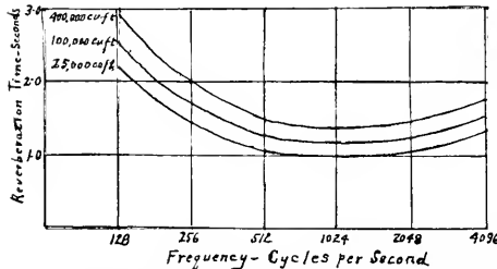
Fig. 1—Optimal reverberation characteristics for rooms of different size which are to be used for both speaking and music.
