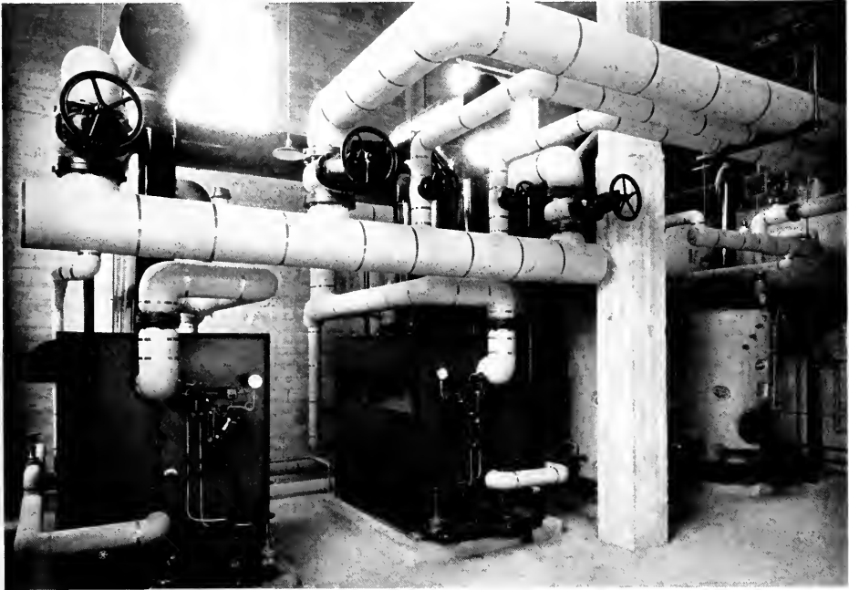
INTERIOR OF BOILER PLANT, ST. BERNARDINE HOSPITAL I. E. Loveless, Architect and Engineer
