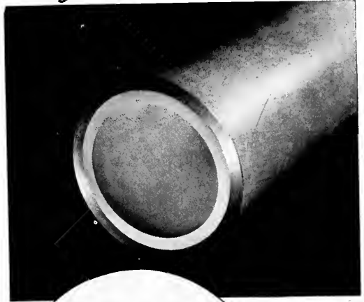
Section of National DUROLINE Pipe coupling and joint. (Note special highly corrosion-resistant joint compound on end of pipe and on threads.)
