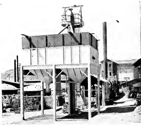
ROTARY KILN AND HOT STORAGE BIN AT GRAVELITE PLANT, POINT RICHMOND
