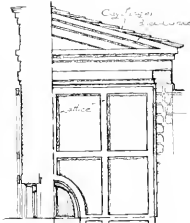
Cornice & Eave Detail
