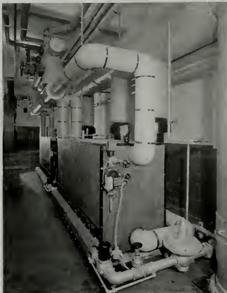
GAS FIRED BOILER PLANT IN SUNKIST BUILDING, LOS ANGELES
