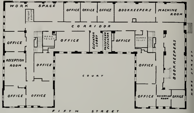
DETAIL SUNKIST BUILDING, LOS ANGELES Walker and Eisen, Architects
