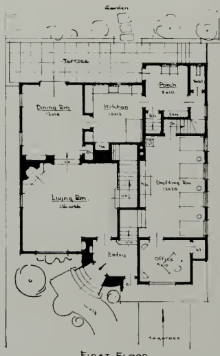
PLANS, STUDIO-RESIDENCE OF F. FREDERIC AMANDES, SAN FRANCISCO
