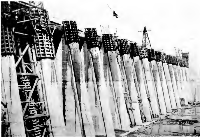
A recent photograph of the power-house dam, across the river channel on the Oregon side. The view is of the upstream face; during construction the water of this channel has been diverted. The power-house at this point will generate 115,000 horsepower, or 86,000 kilowatts; later this output may be doubled.
