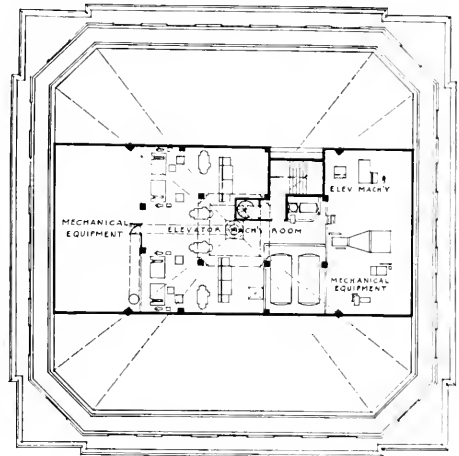
LAYOUT FOR MECHANICAL EQUIPMENT, COURT HOUSE, TWELFTH FLOOR
