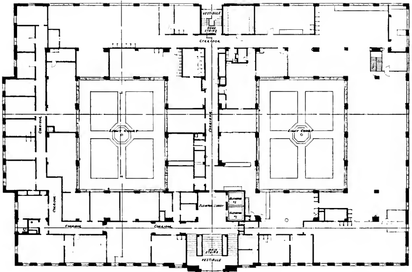
GROUND FLOOR PLAN shows a width of 226 feet 6 inches and depth of 146 feet, providing 26,200 square feet of floor space, and two light courts each 48 feet wide and 61 feet deep.
