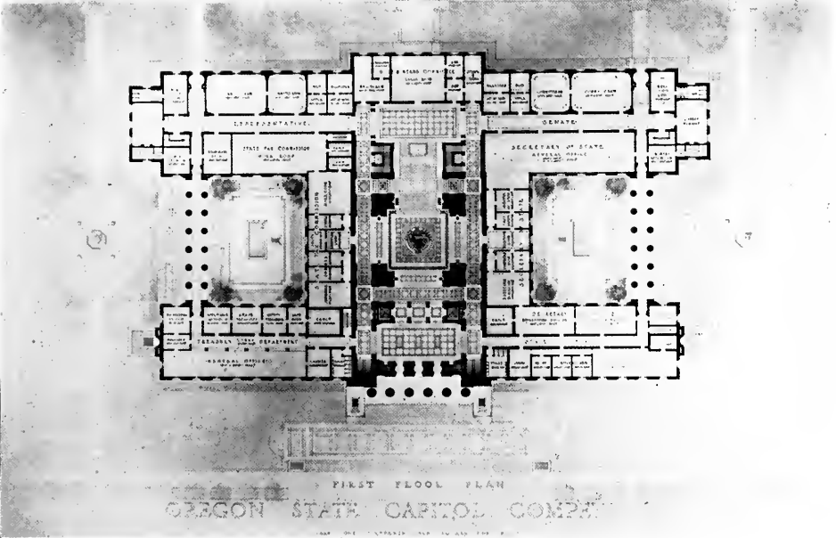
FIRST FLOOR PLAN, OREGON STATE CAPITOL BUILDING W. P. Day, Architect
