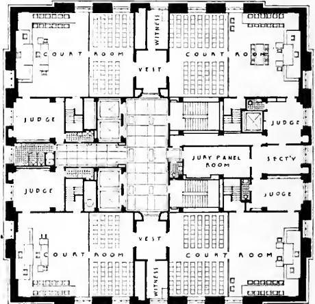
TYPICAL INTERMEDIATE COURT ROOM FLOOR (Fourth, Sixth and Eighth)
