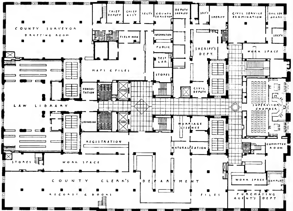
SECOND FLOOR PLAN, COURT HOUSE AND HALL OF RECORDS, OAKLAND, CALIFORNIA
