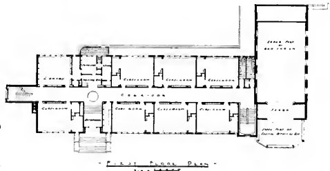
PLANS, LAWTON SCHOOL BUILDING, SAN FRANCISCO Dodge A. Riedy and Chas. E. J. Rogers, Architects
