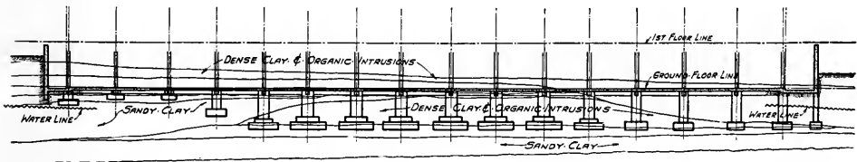
SECTION THRU FOUNDATIONS
