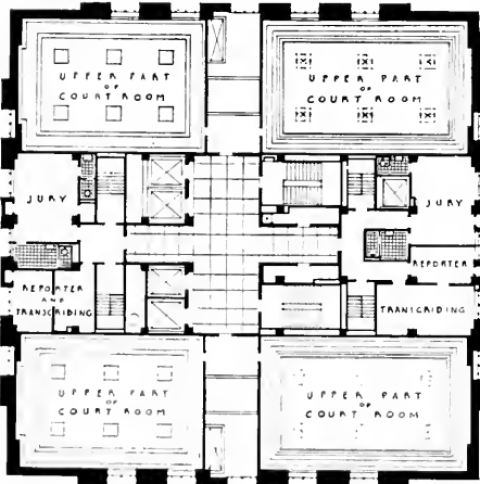
TYPICAL COURT ROOM FLOOR (Third, Fifth and Seventh)
