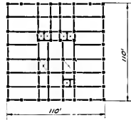
PLAN AT 7TH FLOOR STEEL
