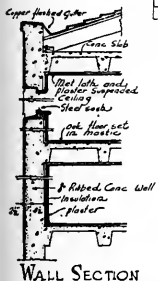
WALL SECTION
