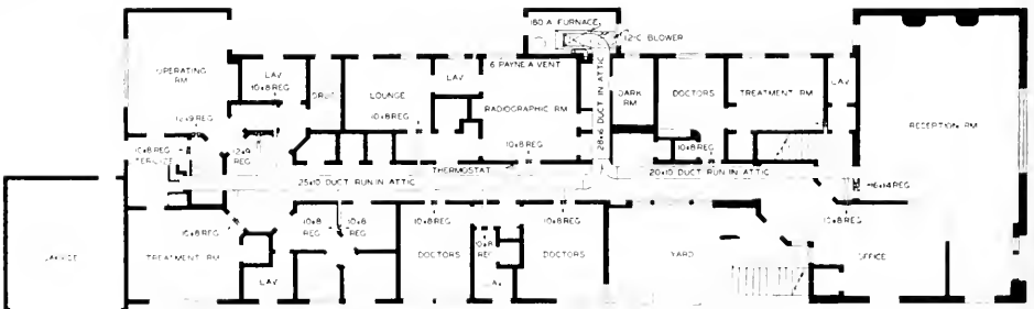
GROUND FLOOR PLAN, DR. F. J. GASPARD MEDICO-DENTAL BUILDING
