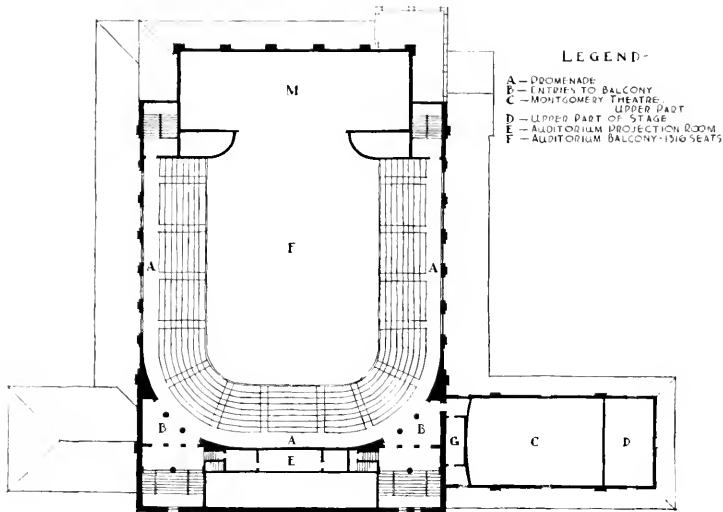
BALCONY PLAN OF BALCONY FLOOR, MUNICIPAL AUDITORIUM, SAN JOSE Binder and Curtis, Architects
