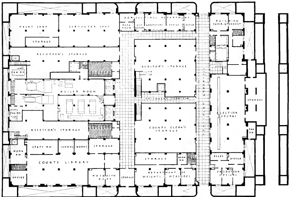
GROUND FLOOR PLAN, COURT HOUSE AND HALL OF RECORDS, OAKLAND, CALIFORNIA
