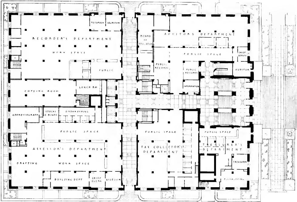
FIRST FLOOR PLAN, COURT HOUSE AND HALL OF RECORDS, OAKLAND, CALIFORNIA
