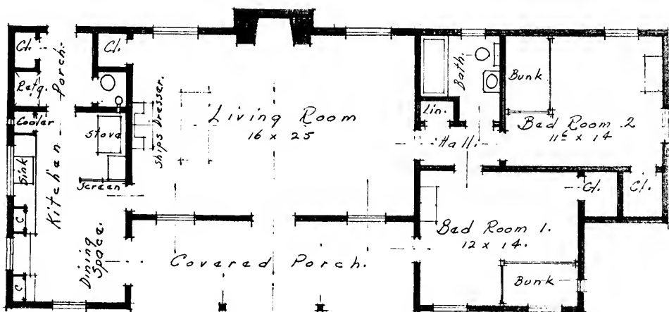
Floor Plan. Scale \frac{1}{8}'' = 1'-0''
