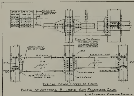
Fig. 1—Typical connection of girder to column
