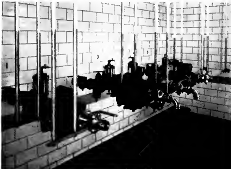
Government Cellar contains four 100-barrel and eleven 250-barrel glass lined tanks. The Wall Units are Kraftile Ceramic Glazed, Cellular, they are ideal for a refrigerated room like this. Kraftile Vitreous 8 x 8 Quarry Tile is used to finish the floor here, in the Meter Room, and the entire working area of Machinery Hall. 13,300 square feet were used—the largest quarry tile installation in San Francisco last year
