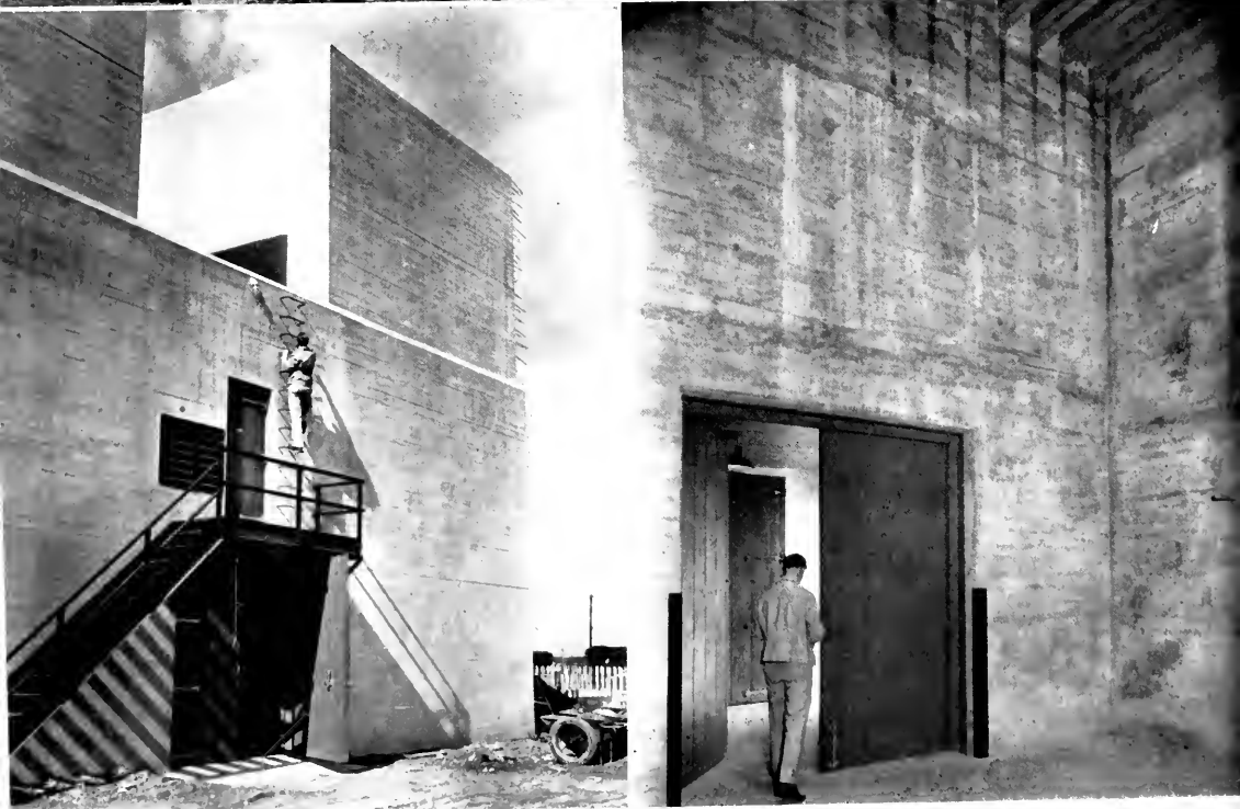
(Top) Exterior view of test stand building. Inlet stacks for the four test cells are on the corners of the structure; outlet stacks in the center each serve two test cells. (Above—left) Exterior view of inlet stacks. (Above—right) Interior view of test cell, showing height from the cell floor that sound-absorbing baffles of Fiberglas pads are installed in an inlet stack.
