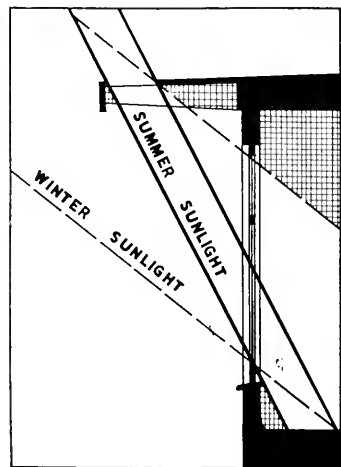
HOUSE IN MENLO PARK, CALIFORNIA Mario Corbett, Architect
