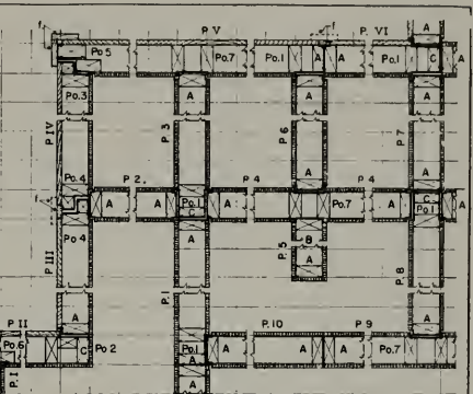
TYPICAL INTERIOR AND EXTERIOR PANEL JOINTS
