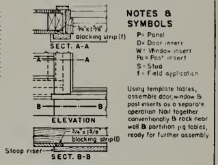
TYPICAL INTERIOR AND EXTERIOR PANEL JOINTS
