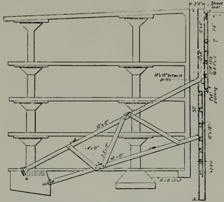
Timber braces for the steel piles and steel tierads to resist vertical component of thrust
