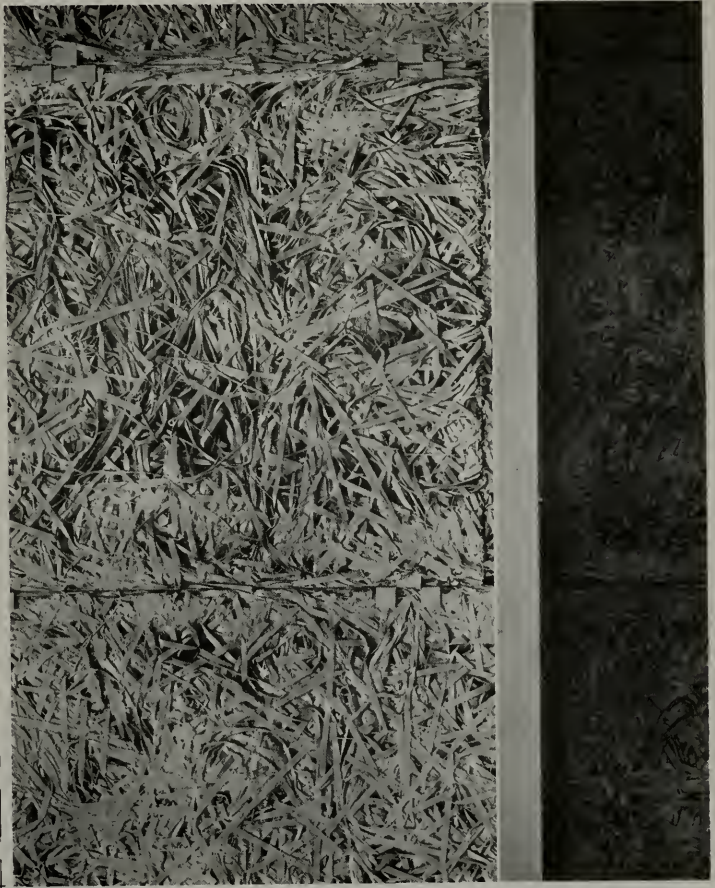
DETAIL OF WALL AND ROOF CONSTRUCTION, INDUSTRIAL PLANT, WITH CLOSE-UP OF THERMAX WALL FINISHED WITH CEMENT PAINT
