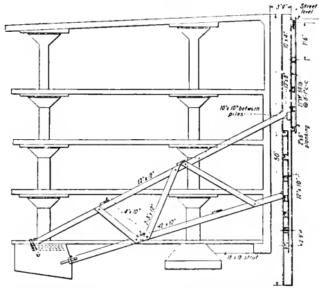
Timber braces for the steel piles and steel ties to resist vertical component of thrust
