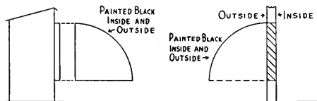
Elevation section and floor plan of factory equipped with blackout ventilation
