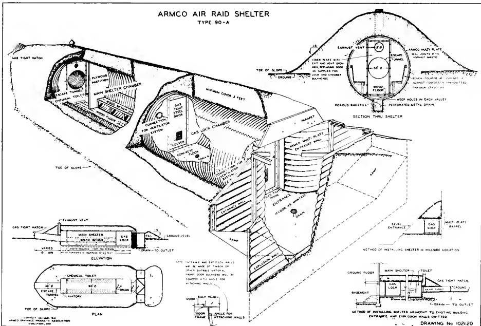
This Armo iron air-raid shelter is 50 ft. long and 7 1/2 ft. high and will accommodate 50 persons. Four unskilled workmen can erect the shelter with simple tools in a few hours.
