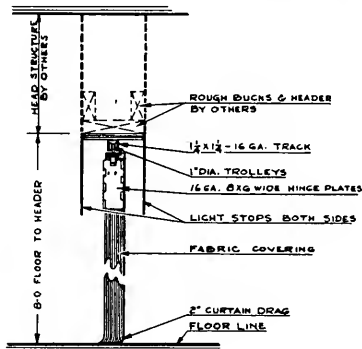
VERTICAL SECTION
