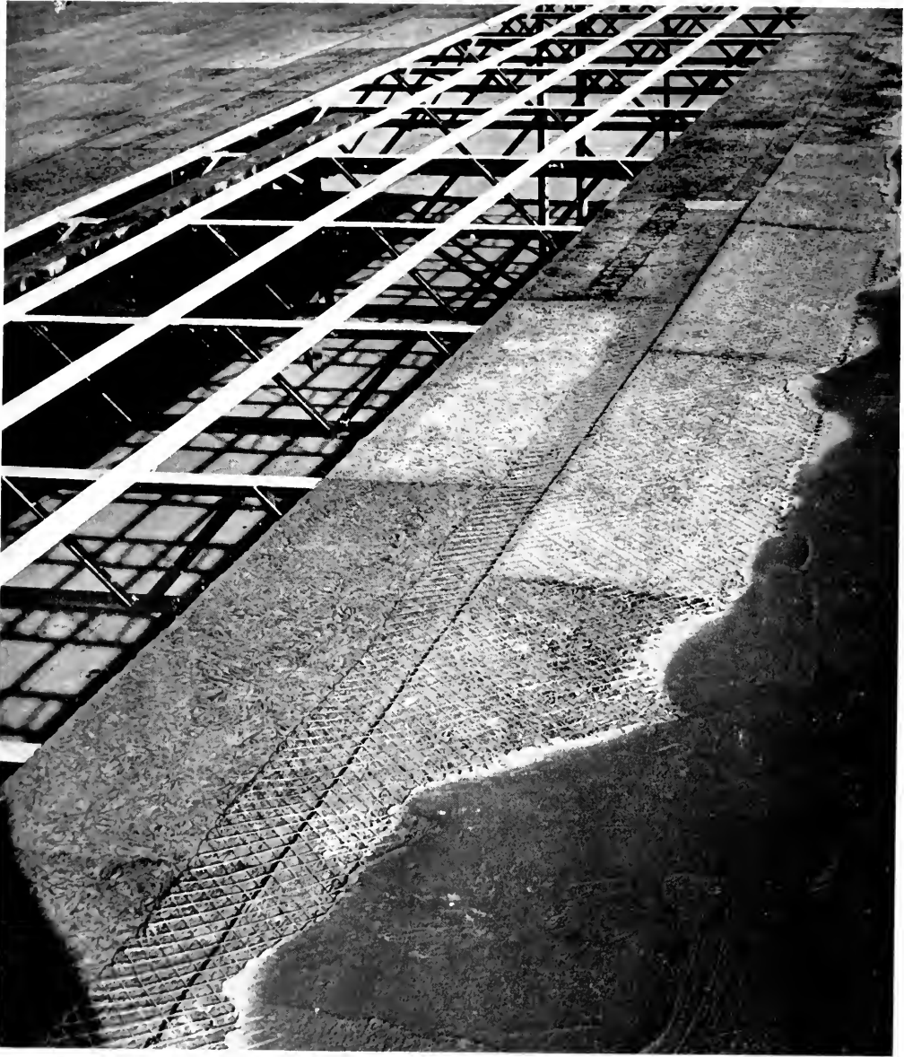
ROOF CONSTRUCTION OF INDUSTRIAL PLANT, SHOWING STEEL, THERMAX, WIRE AND CEMENT TOPPING
