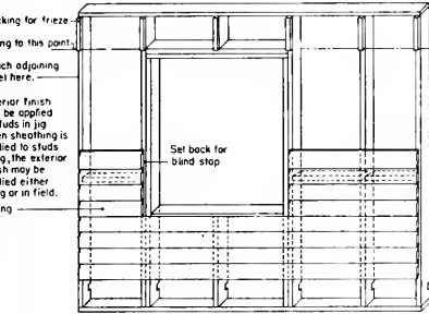
EXTERIOR WALL PANEL FRAMING
