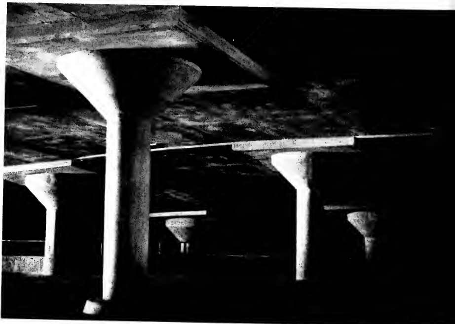
Irregular shaped columns, some 50 in number, serve as floor supports, formed in metal and installed by the Steel Form Contracting Company
