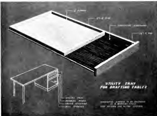
DRAWER-TRAY FOR DRAFTING UTILSIES DESIGNED FOR STUDENTS' WORK
