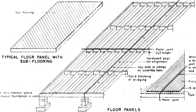
FLOOR PANELS
