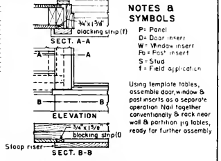
DETAILS OF EXTERIOR DOOR SILL & FRAME
