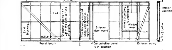
EXTERIOR WALL PANEL FRAMING
