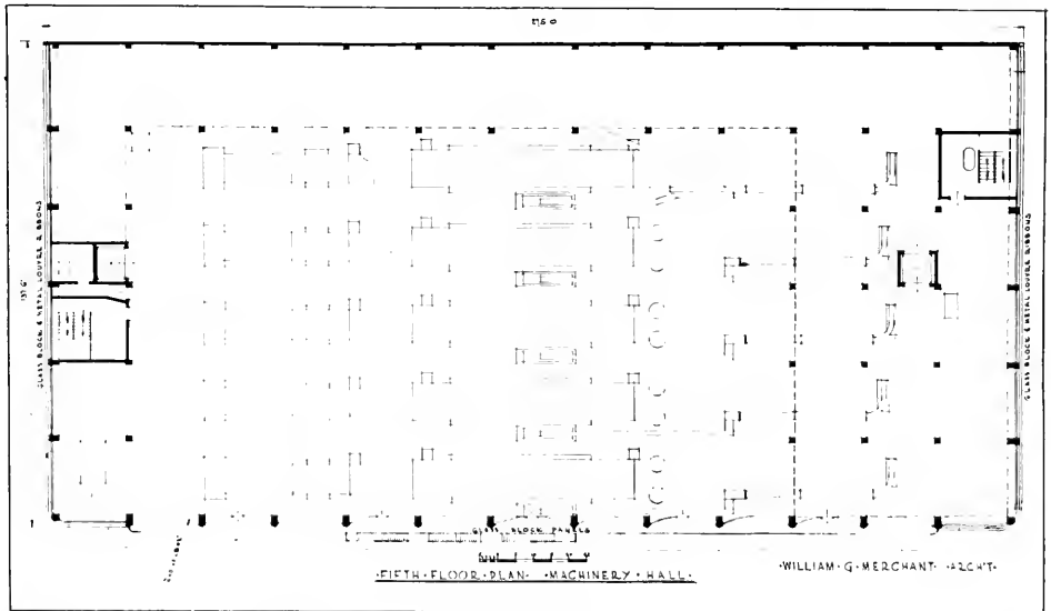
PLAN OF FIFTH FLOOR, ACME BOTTLING PLANT, SAN FRANCISCO
