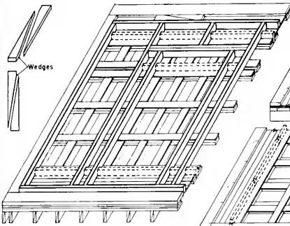
This drawing indicates framing for wall panel in the jig
