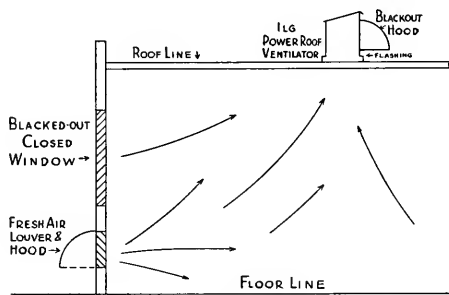
ELEVATION SECTION
