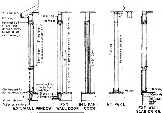
EXTERIOR WALL PANEL FRAMING
