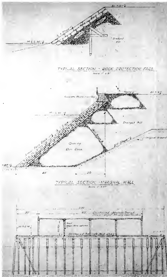
TYPICAL SECTIONS, PROPOSED TRANS-PACIFIC AIR BASE
