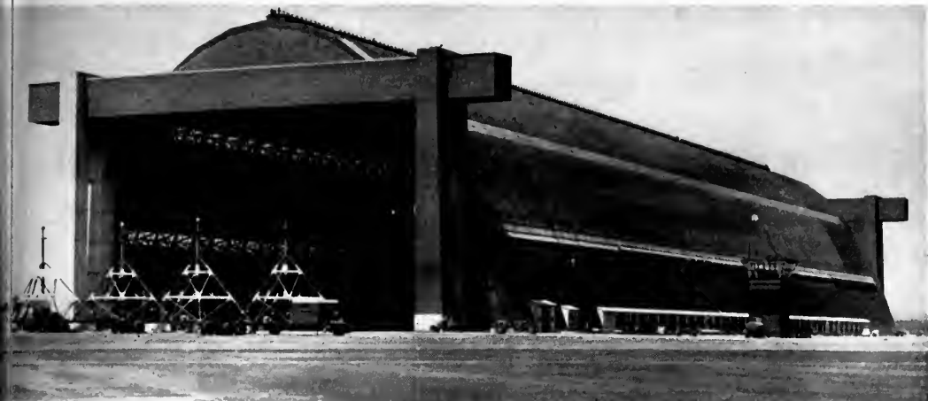
Wooden blimp hangar at the Naval Air Base, Santa Ana, California, is 171 feet high, and has a clear span across of 237 feet, largest ever erected.
