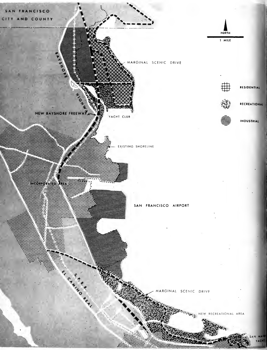
PLAN FOR COORDINATED BAY SHORE DEVELOPMENT (Prepared by the San Mateo County Planning Commission)
