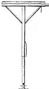
Top: Adjustable Tee-Post
