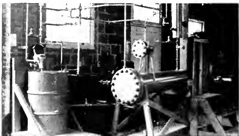
• Autoclave for Pressure Treating Woods with chemicals and preservatives, Automatic Mixer at left.
