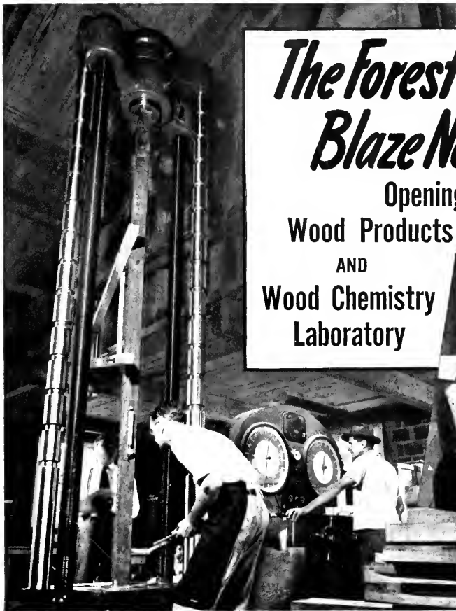
↑ TECO Chemistry Laboratory. TECO chemists are here shown working on lignin derivatives. ← 200,000 lb. Baldwin-Southwark testing machine in the TECO Shop. Material undergoing test is a small wood column being tested in compression.
