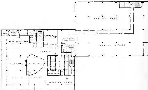
13th Floor Plan of Textile Building
