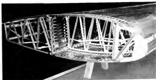
Section of outer wing panel all stainless steel airplane.
