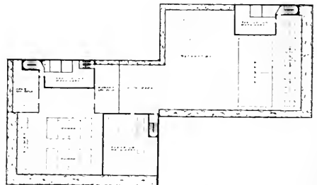
Roof Plan of Textile Building
