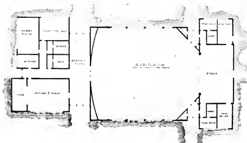
FLOOR PLAN of new Auditorium.
