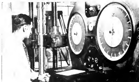
• 200,000 lb. Baldwin-Southwork Hydraulic Testing Machine for tension compression and bending tests on wood.
