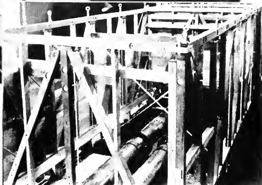
Cooling tower framing with outer sheathing partly applied. Note TECO Connectors are used for joining framing at corners and diagonals. Tower built by Foster Wheeler Corporation, New York. →
